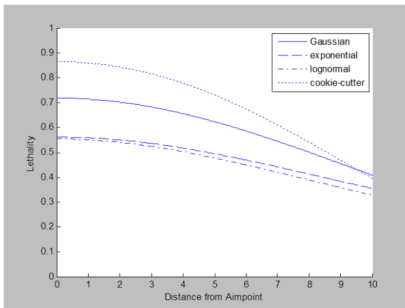
Figure 32: Lethality Function
