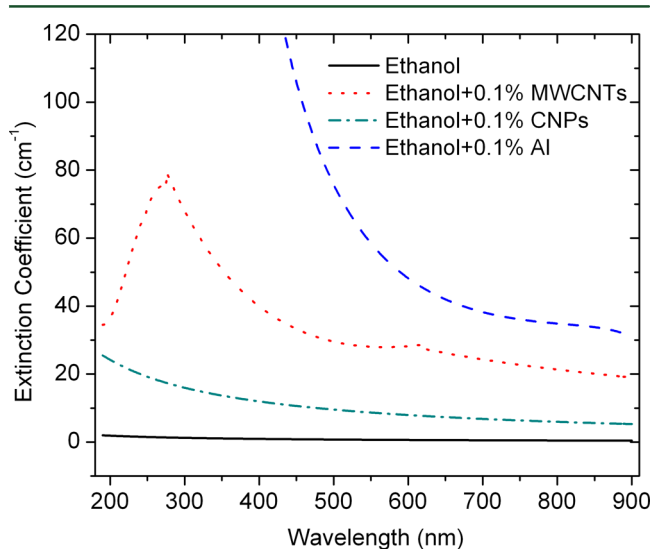
Figure 8. Calculated extinction coefficient of pure ethanol and nanofluids with the addition of Al particles, CNPs, and dispersible MWCNTs.
