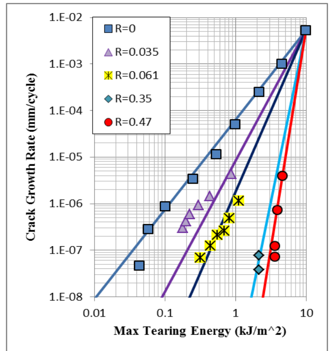
Figure 7: Traditional method: experiments vs. fitting.
