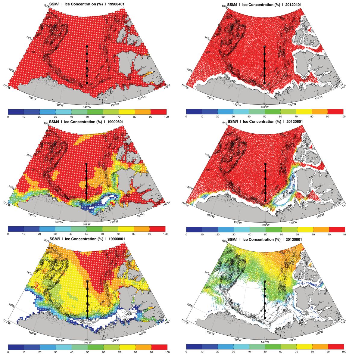
Figure 1. SSM/I ice cover for April, June, and August (top, middle, and bottom) for 1990 (left) and 2012 (right). Prior to the recent period of sea ice decline, the MIZ rarely extended beyond the Alaska slope. More recently, the seasonal MIZ develops in July and retreats rapidly northward, leaving large expanses of open water over the Alaska slope and into the deep Beaufort Sea.
