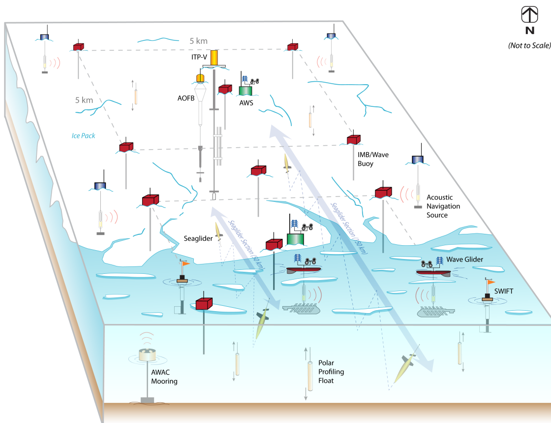
Figure 5. Ice-edge and ‘5-dice’ IMB/WB sub-array configuration, depicting oceanographic sampling by floats and gliders beneath the ice and by various ice-based instruments that penetrate through the ice. Gliders conduct sections that extend from full ice cover, through the MIZ, and into open water. Wavegliders and SWIFT drifters sample within the MIZ and the open water to the south.
