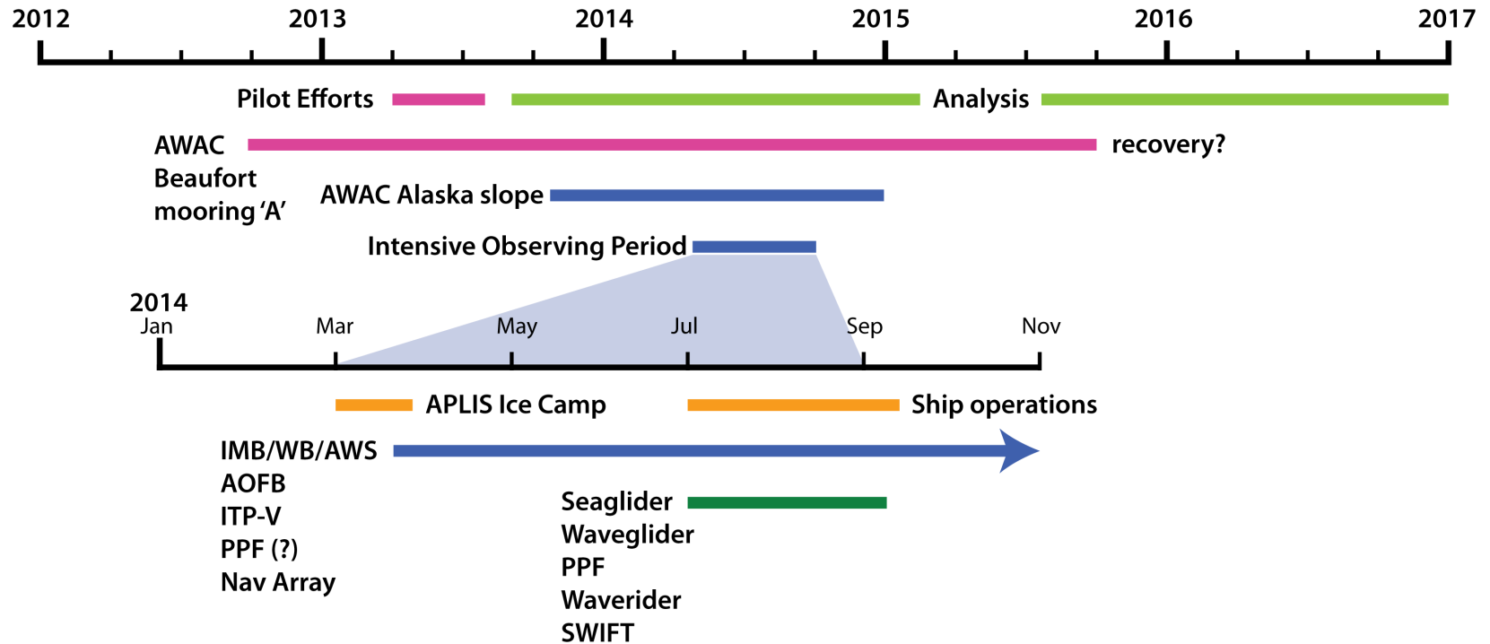
Figure 3. Timeline of the five-year MIZ Program. Magenta and blue bars in the upper timeline (2012–2017) mark two extended deployments of subsurface AWAC moorings. The lower (expanded) timeline describes the 2014 intensive observing period, with orange bars marking the ice camp and ship operations intervals, the blue bar indicating the (open-ended) sampling by ice-based platforms and the green bar delineating sampling by mobile and drifting platforms.
