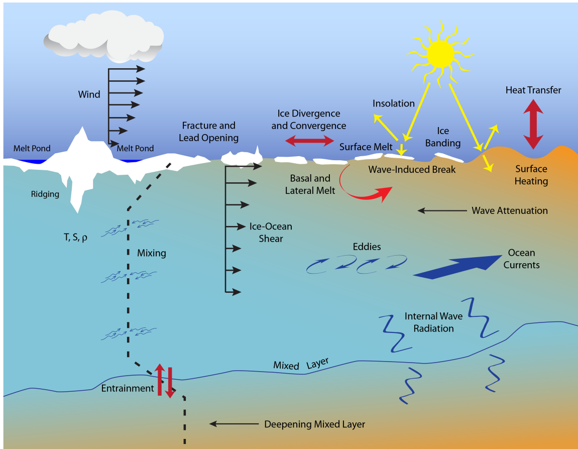
Figure 2. Atmosphere, ice, and upper ocean processes in the MIZ. Ice cover modulates penetration of solar radiation and isolates the upper ocean from direct wind forcing, but increasing open water within the MIZ, and the proximity of large expanses of open water immediately to the south, permits more direct connection with the atmosphere. Strong open water swell and surface wave activity attenuates as it enters the MIZ. Likewise, internal waves, submesoscale eddies, and mixing weaken with increasing ice cover. Small-scale windstress curl associated with ice to open water transitions and variations in ice roughness may induce intense secondary circulations that drive rapid vertical exchange. Enhanced mixing and vertical exchange can entrain heat stored below the mixed layer, increasing basal melting of sea ice within the MIZ. In ice-covered regions, local radiative solar warming leads to direct ablation of sea ice and some bottom melt from the radiation penetrating weakly into the ice-covered upper ocean. Open water regions within and south of the MIZ allow increased radiative upper ocean warming and, through lateral advection, accelerated ice melt. These processes are expected to amplify variance at short spatial and temporal scales across the MIZ.
