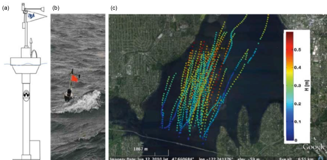
Figure 12. Surface Wave Instrument Float with Tracking (SWIFT) drifter: (a) schematic, and (b) deployed. SWIFTs measure wind speed, wave height [(c) Lake Washington, Seattle], wave directional spectra, air temperature, sea surface temperature, surface currents, and dissipation by turbulence.
