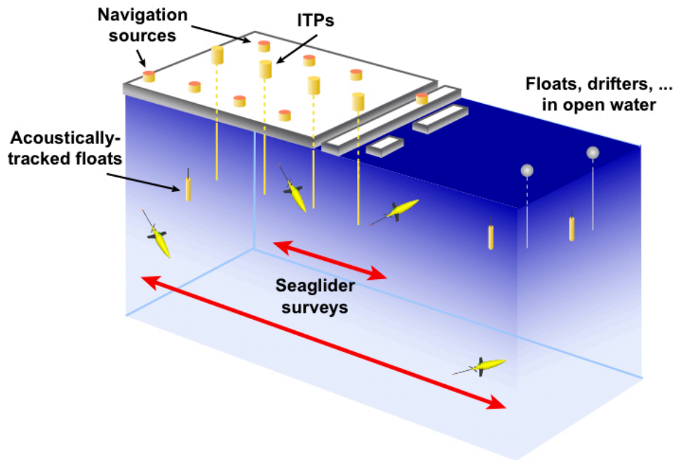
Figure 9. The Mobile MIZ Observing Network. Ice-Tethered Profilers, ice-capable Seagliders, and profiling floats, with an acoustic array providing under-ice geolocation and navigation, provide high spatial and/or temporal resolution ocean measurements in the MIZ. The array follows ice drift and retreat through the melt season. Gliders sample from open water, through the MIZ, and into full ice cover, profiling from the ice–ocean interface to 1000 m depth.
