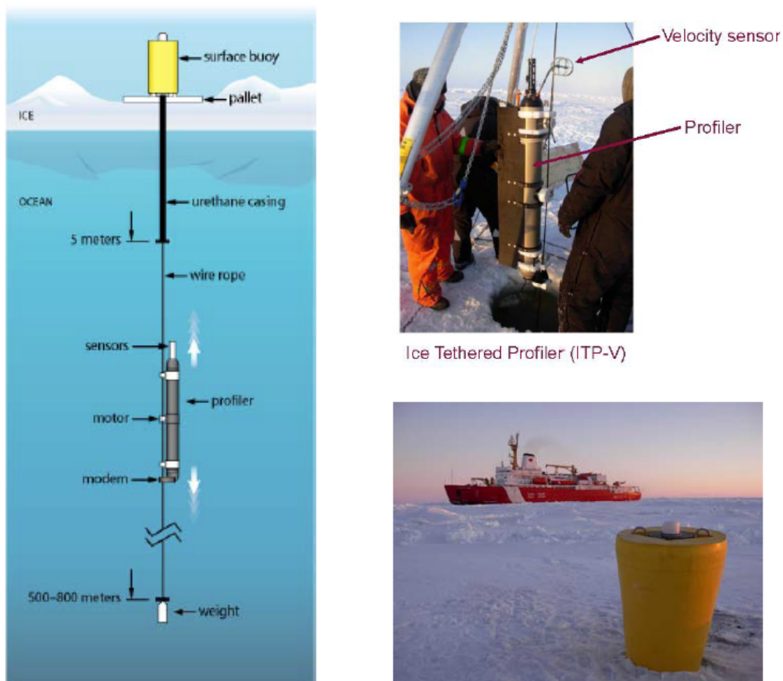
Figure 8. Schematic of the WHOI Ice-Tethered Profiler system (left), the profiler with velocity sensor (ITP-V) prior to deployment (upper right), and the surface expression (lower right).
