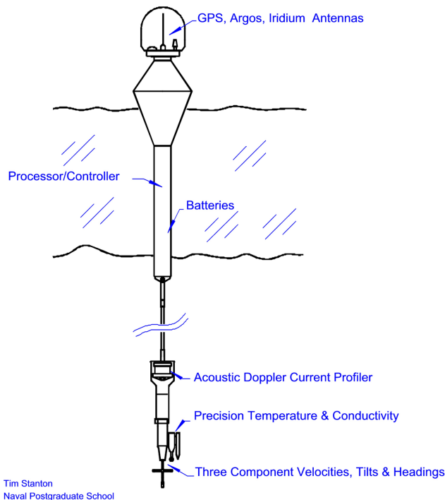
Figure 7. The Naval Postgraduate School (NPS) Autonomous Ocean Flux Buoy (AOFB). A surface buoy sits on the ice supporting an instrument package suspended into the upper ocean by a series of poles from the bottom of the surface buoy. The surface buoy contains processing electronics, GPS and Iridium antennae, and batteries. The instrument package is outfitted with a downward looking 300-kHz Acoustic Doppler Current Profiler (ADCP, RDI Workhorse) and a custom-built flux package. Additionally, the buoys have GPS receivers for measuring position and calculating ice velocity. After installation in the field on selected ice floes, AOFBs maintain twice-daily, two-way communications with a computer running at the NPS.
