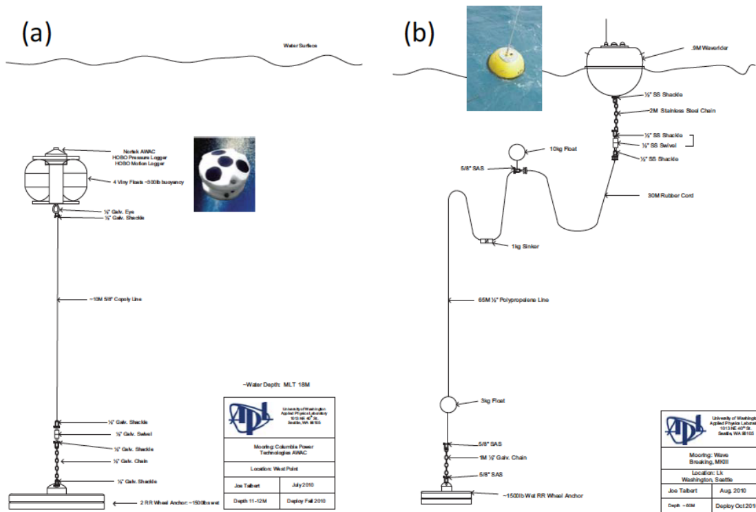
Figure 11. (a) Nortek Acoustic Wave and Current (AWAC) and (b) Waverider moorings. Waveriders may also be deployed in a drifting configuration.
