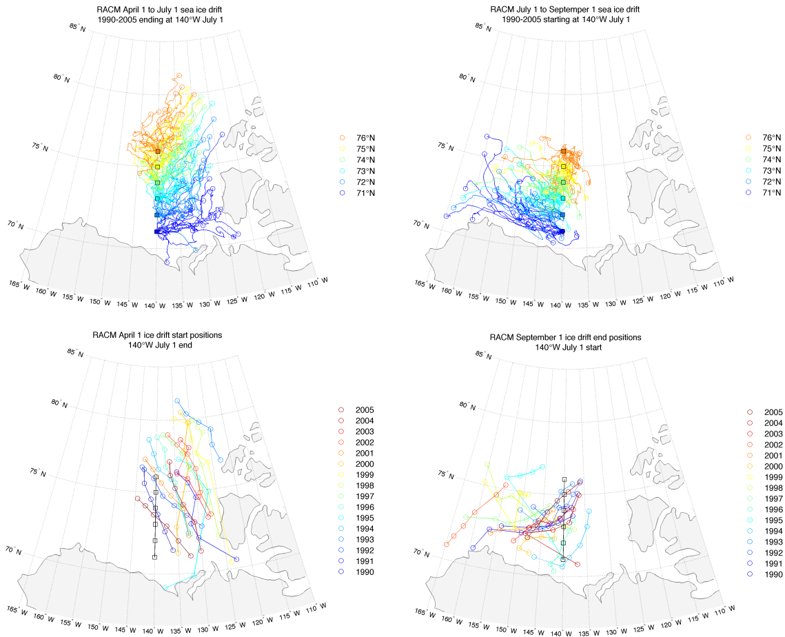
Figure 6. Simulated trajectories (1990–2005) derived from analysis of the Naval Postgraduate School’s fully coupled Regional Arctic Climate Model (RACM). Back-calculated trajectories (upper left) and starting positions (lower left) from the target 70°–76°N, 140°W line from 1 July to 1 April and forward trajectories (upper right) and end positions (lower right) from the target line on 1 July to an endpoint on 1 September.
