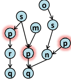
Figure 5.5: Coherence graph. Nodes represent papers (names appear inside). Paths represent coherent chains. Each paper may have multiple corresponding vertices: the highlighted vertices are all copies of paper p .
