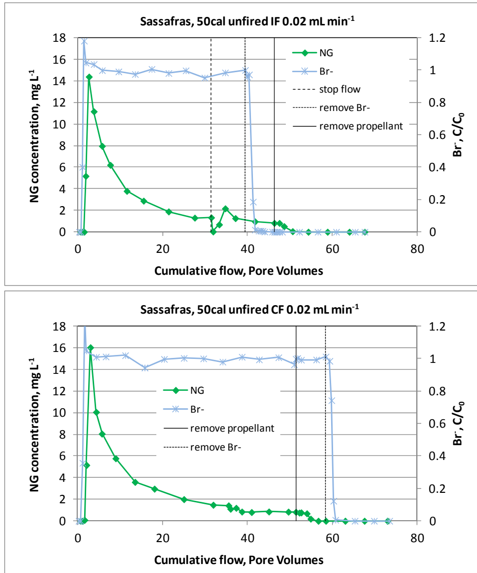
Figure C7. Breakthrough curves for continuous (CF) and interrupted (IF) water flow at 0.02 mL min -1 rate onto unfired and fired 0.50-cal. propellants in SassafRAS soil. The solid vertical line indicates when the propellant was removed from the soil surface.
