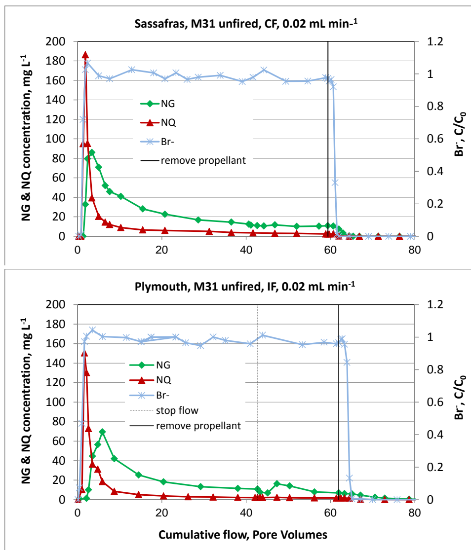
Figure 44. Breakthrough curves for continuous (CF) and interrupted (IF) water flow at 0.02 \text{ mL min}^{-1} rate onto unfired M31 propellant in Sassafras and Plymouth soils. Breakthrough of NG happened later in Plymouth compared to Sassafras soil indicating greater adsorption of NG.
