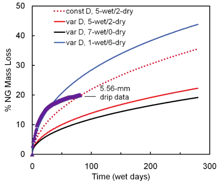
Figure 36. FEM predictions for constant and variable diffusivity with 5-day wet/2-day dry cyclic wetting (red curves) compared with data for 5.56-mm unfired grains in drip test and FEM predictions for variable diffusivity and continuous wetting 7-day wet/0-day dry and cyclic 1-day wet/6-day dry.
