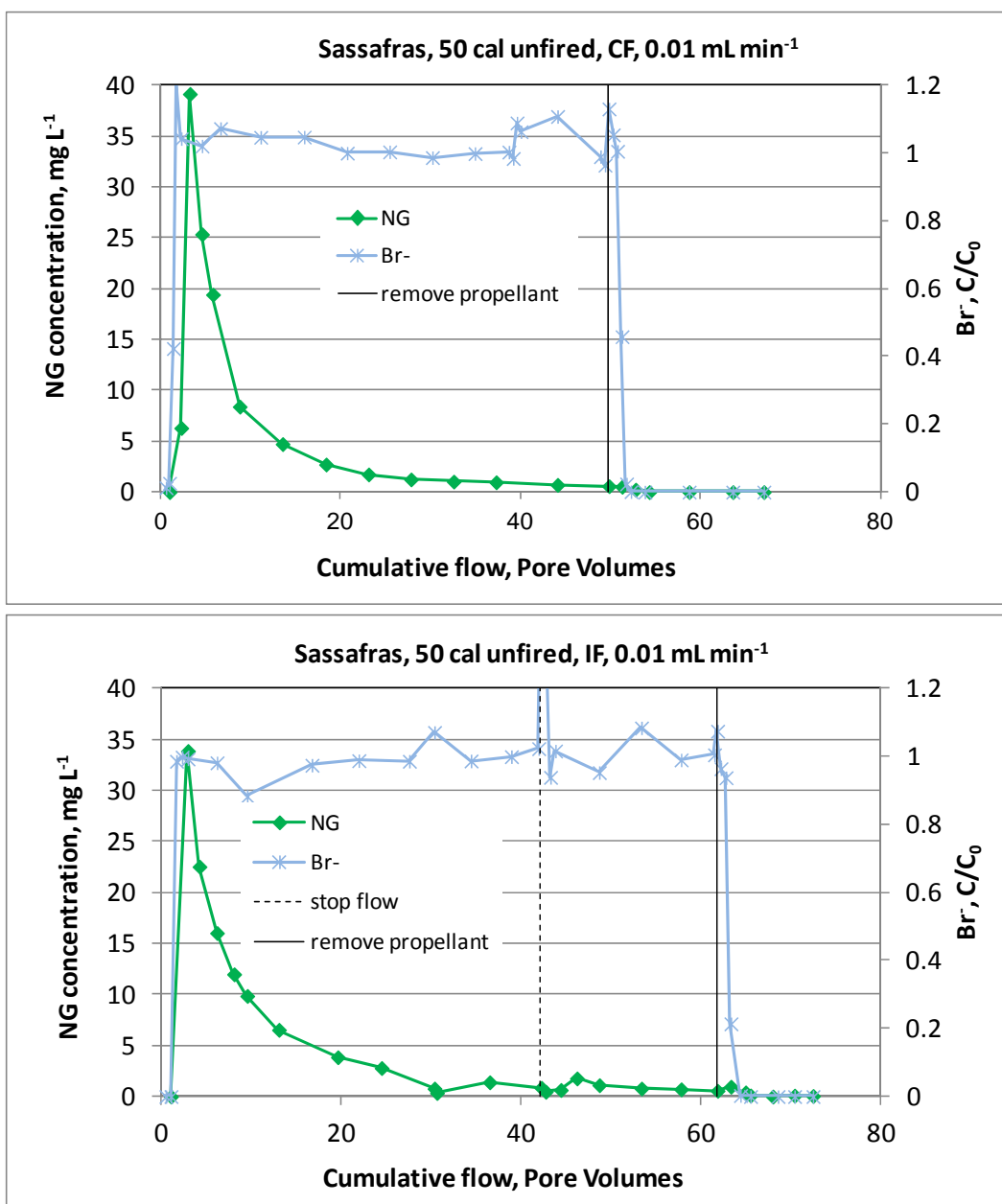
Figure C5. Breakthrough curves for continuous (CF) and interrupted (IF) water flow at 0.01 mL min -1 rate onto unfired and fired 0.50-cal. propellants in Sassafra soil. The solid vertical line indicates when the propellant was removed from the soil surface.
