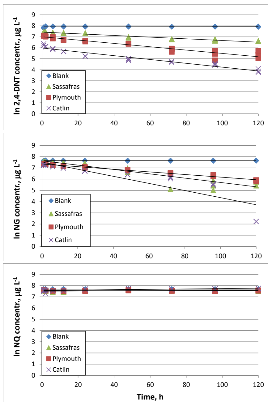
Figure 38. The natural logarithm of 2,4-DNT (top), NG (center), and NQ (bottom) in suspensions of Sassafra, Plymouth, and Catlin soils concentrations plotted as a function of time. Also plotted is our control that contained no soil. The slope of regression line is the transformation rate ( k ) (Table A2).
