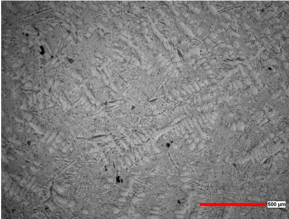
Figure 3 Microstructure of the base alloy A380 cast under similar conditions (50×). Dendritic networks of primary Al, primary Si, possible \text{Al}_5\text{FeSi} and \text{Al}_{15}(\text{Fe,Mn})_3\text{Si}_2 , and porosity are observed.
