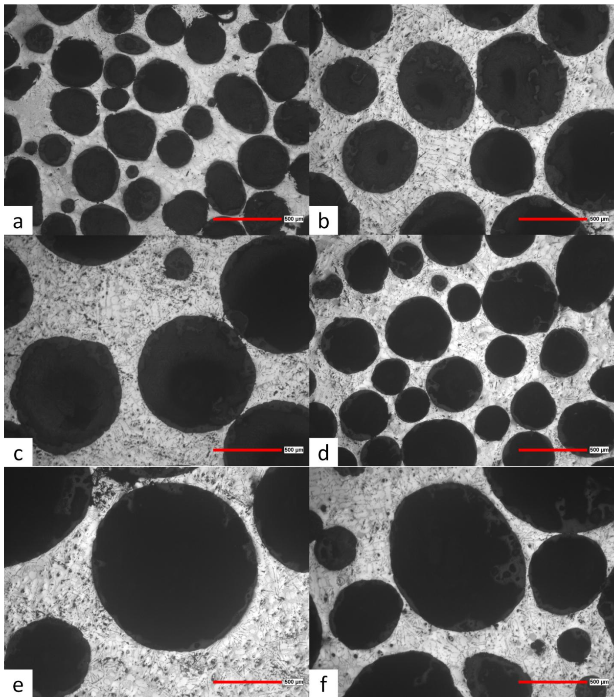
Figure 4 Representative microstructures of A380- \text{Al}_2\text{O}_3 syntactic foams containing hollow spheres with diameters a) 0.212-0.425 mm, b) 0.425-0.85 mm, c) 0.85-1 mm, d) 0-0.5 mm, e) 1-2 mm, f) 0-2 mm.
