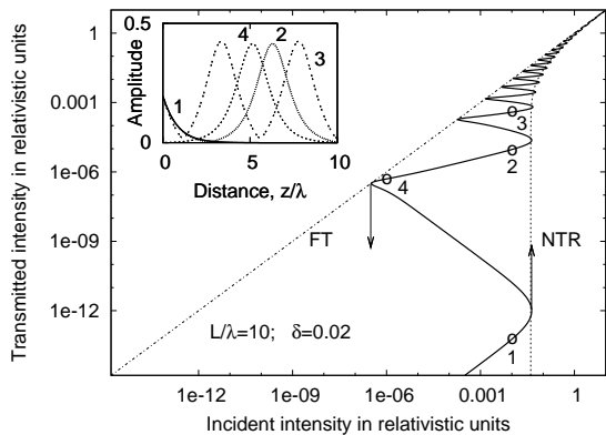
FIG. 1: Hysteretic transmission of light through a plasma layer of thickness L . FT and NTR are full transparency and near total reflection limits. Points 1, 2, 3 mark a linear evanescent wave, 1-st, and 2-nd upper stable states respectively, and 4 – a R-wave sustained by a very low pumping. Arrows indicate direction of jumps within the lowest hysteretic loop. Inset: spatial amplitude profiles of waves corresponding to points 1-4 in the main plot.
