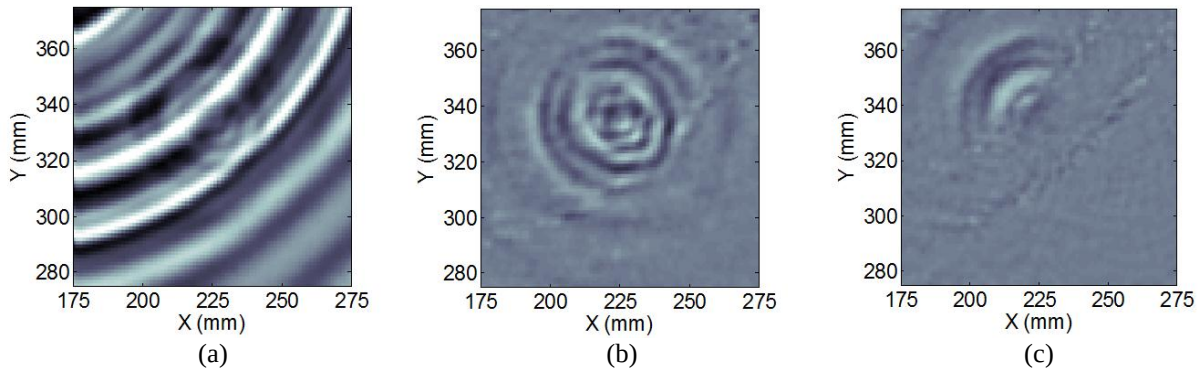
FIGURE 2. Analysis of waveforms in a region around Hole H3 where data were windowed in space over the zoomed region, in time from 0 to 50.6 \mu s, and in frequency from 0.2 MHz to 0.3 MHz. Snapshots of (a) the original wavefield, (b) after application of the time domain source removal method, and (c) after removing the out-going waves in the \omega - k_r domain (applied to the original wavefield).
