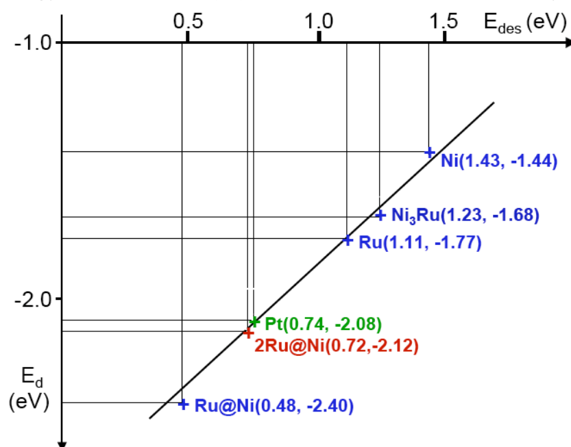
Fig. 1 reports in graphical form the calculated Hydrogen Desorption Energy E_H^{des} and the Center of mass Energy of the d band ( E_d ) for the various tested metal systems.
