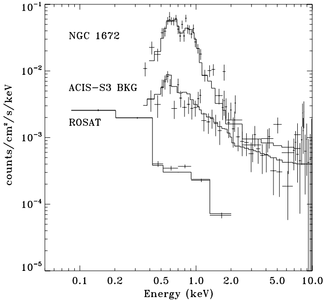
Figure 7. Chandra ACIS spectral data and fit for the diffuse galaxy spectrum, the Galactic foreground/extragalactic background, and RASS data. The ACIS-S1 background spectrum is not shown for clarity.
