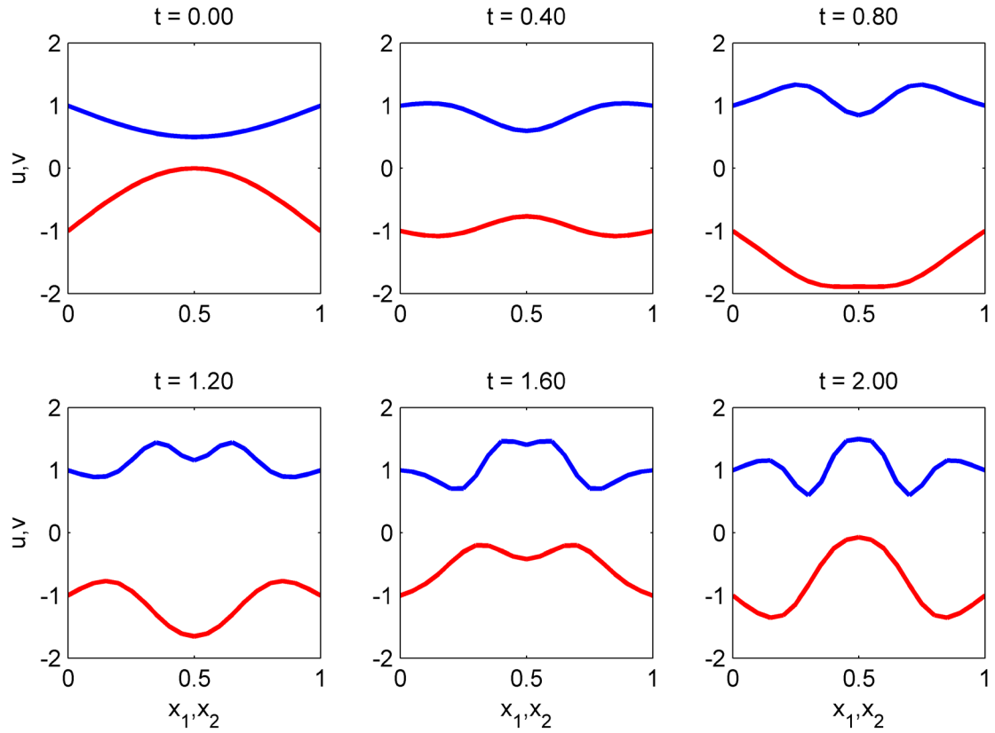
Figure 5. Projection View of the Response of v(x_1, x_2, t) (blue line) and u(x_1, x_2, t) (red line) Along the Same Axis for Case 2 at Time Snaps t = 0.0, 0.4, 0.8, 1.2, 1.6, and 2.0
