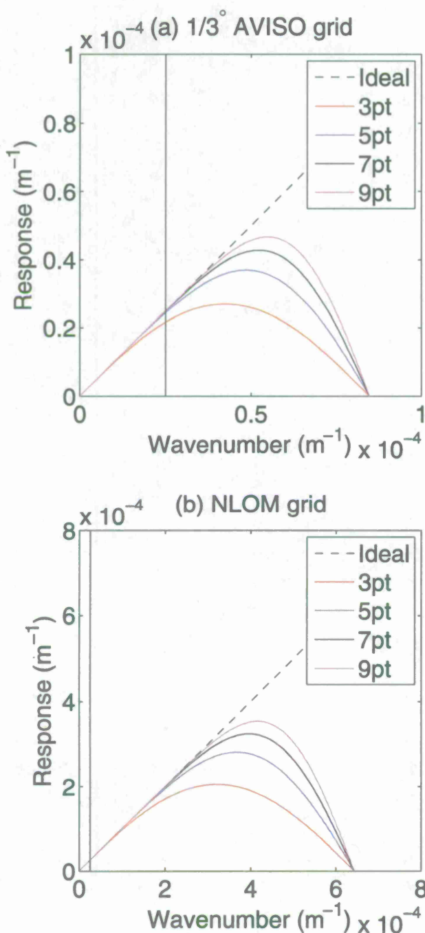
Figure 2. Response of an ideal differentiator and of 3-, 5-, 7-, and 9-point stencils, as a function of wave number, on (a) 1/3° AVISO grid and (b) NLOM grid. The grid spacings used for Figures 2a and 2b are 37 and 4.9 km, respectively, and the response is the absolute value |A| of the eigenvalue of the von Neumann analysis. See text for more details. Vertical lines are drawn at the wave number (40 \text{ km})^{-1} , corresponding approximately to the 2–3° wavelength resolution limitation of the AVISO sea surface height fields.
