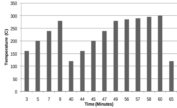
Figure 15: Temperature stress profile
