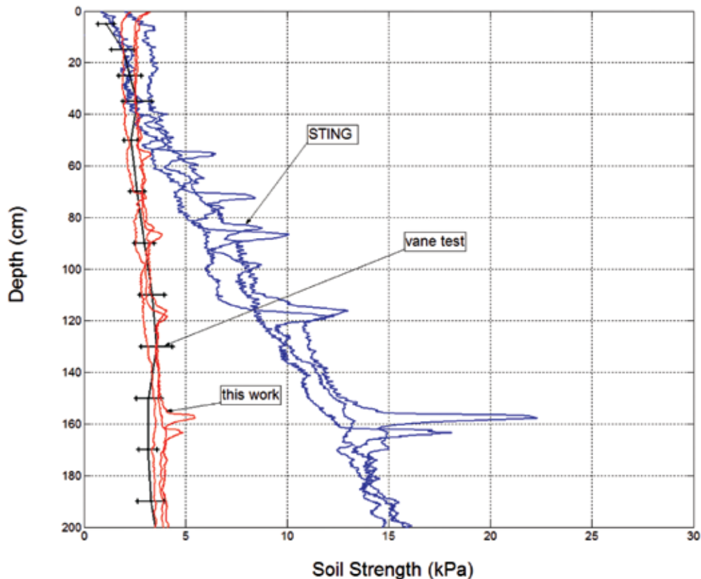
FIGURE 6 STING-processed (blue) and FLAC3D-computed (red) undrained shear strength computation from a location in the Gulf of Mexico, compared with the lab-measured vane test results (black solid lines with error bars representing the standard deviation).
