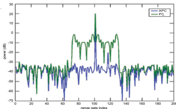
Plot of received signal power after pulse compression processing for a series of range gates. Using traditional pulse compression (green), the sidelobes of the high RCS target at range gate 100 mask the presence of the low RCS target at range gate 120. The APC process (blue) suppresses the sidelobes, allowing detection of the smaller target.
