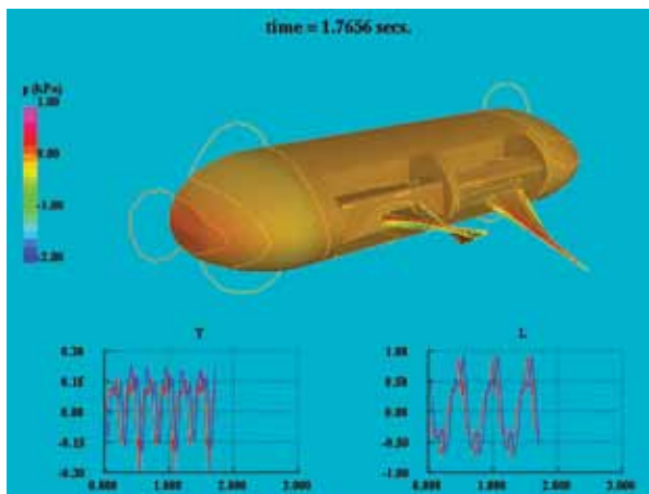
Flow past an unmanned underwater vehicle (UUV) propelled by flapping fins with controlled deformation.
