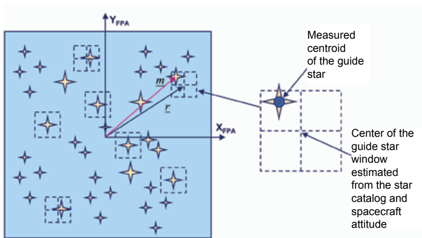
FIGURE 2 Guide stars and their windows in the focal plane array (FPA).
