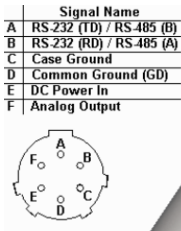
PPTR depth sensor wiring pin out.
