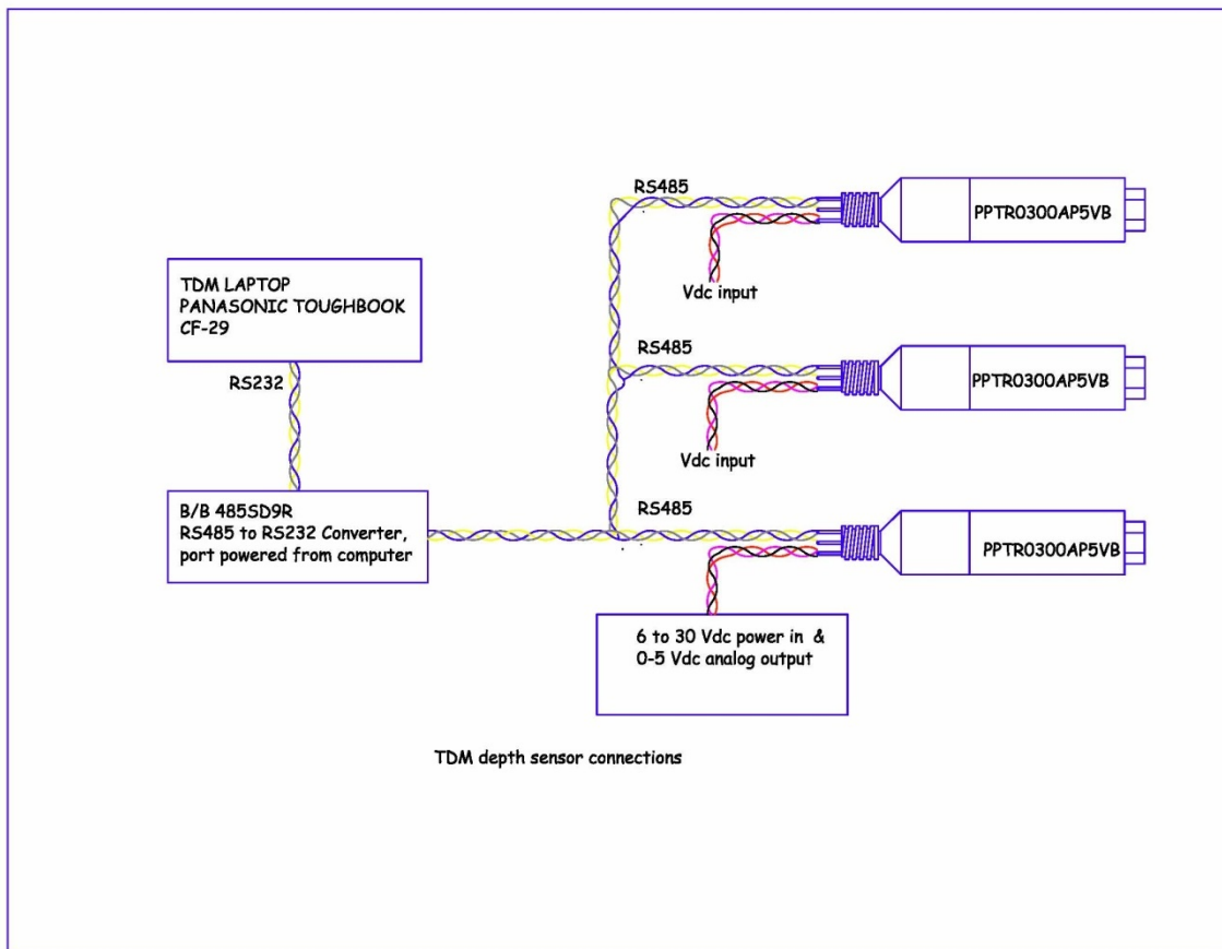
PPTR depth sensor wiring pin out.
