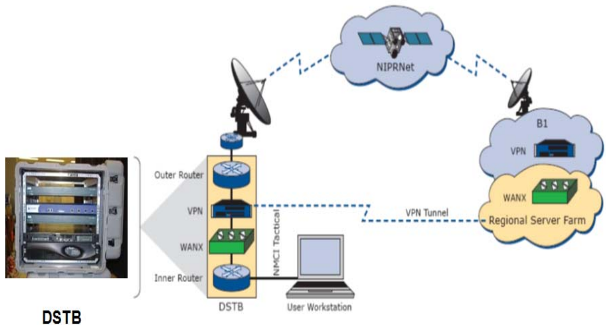
Figure 4. DSTB Architecture (From Hewlett-Packard Development Company, 2010)
