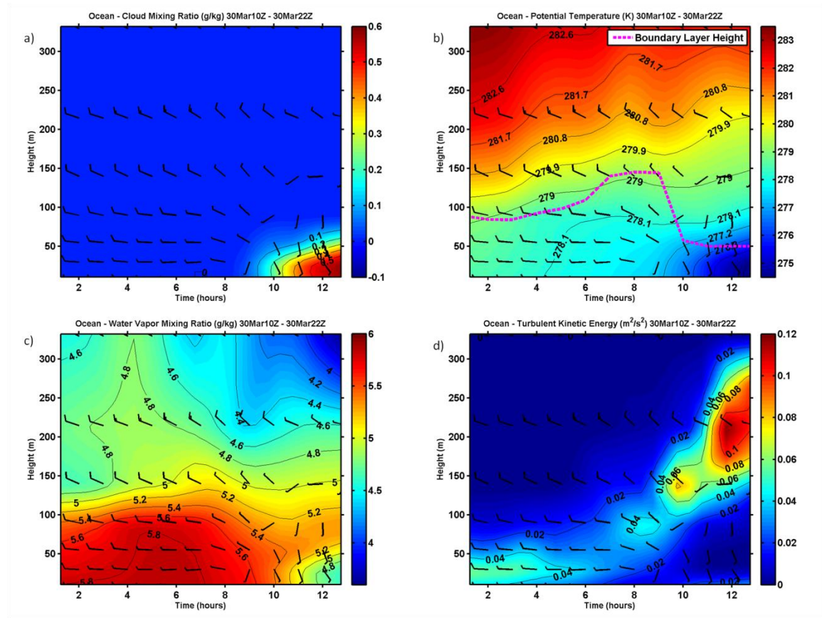
Figure 19. Vertical cross-section plots along the trajectory ending at point O from 30 March/10Z to 30 March/22Z. a) q_c ; b) potential temperature with BL height; c) q_v ; d) TKE. Wind barbs represent the wind speed and direction of the flow in knots.
