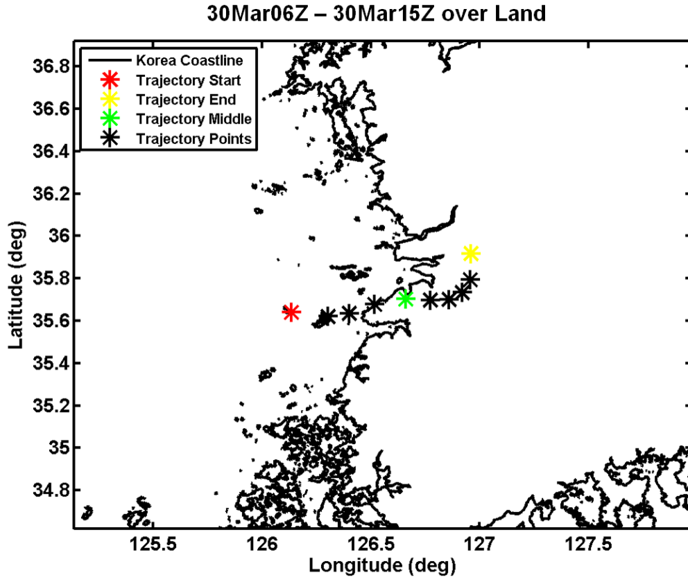
Figure 24. Point L - The forward trajectory path of the air beginning to the west (red star) and ending at the point of interest when the fog began (yellow star).
