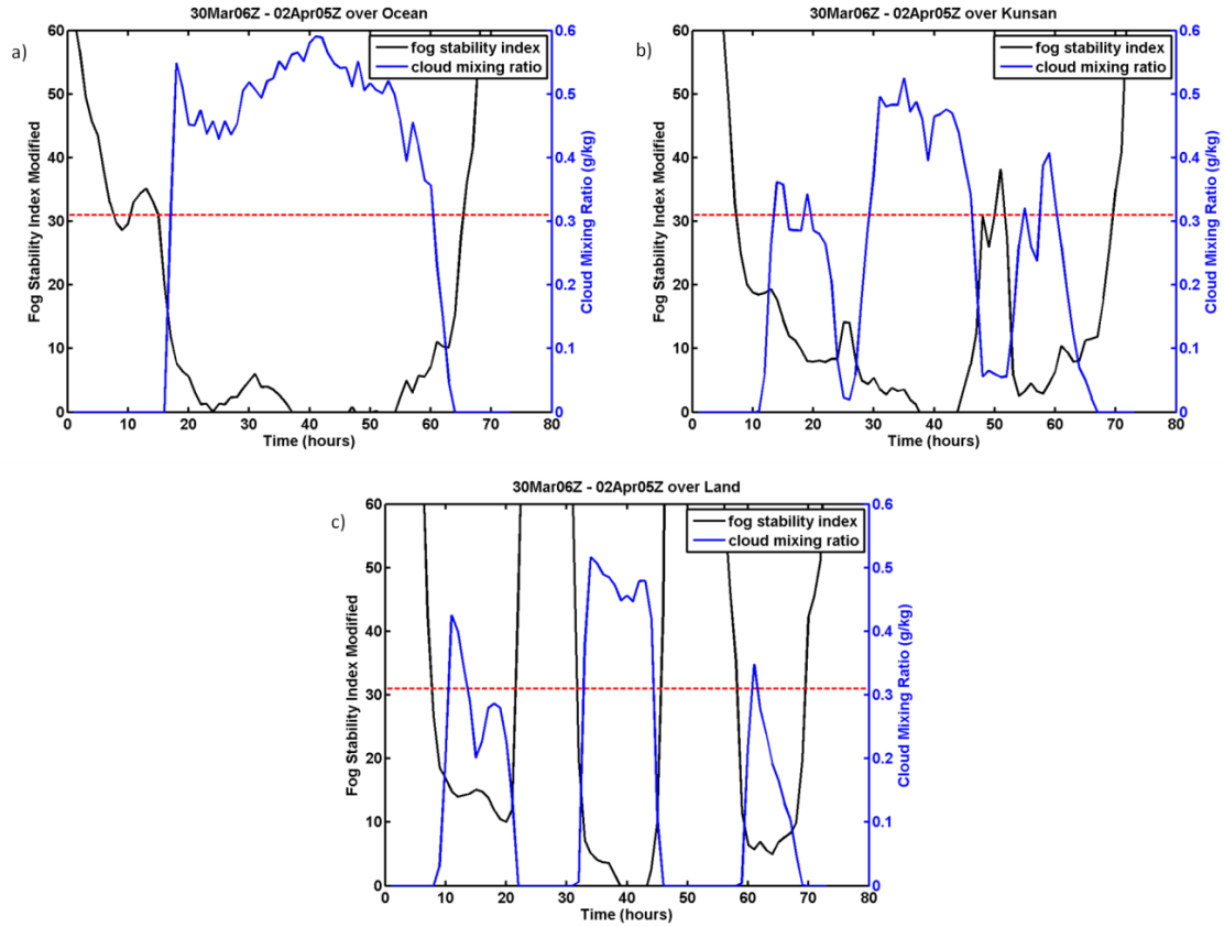
Figure 36. Time series analysis from the points of interest comparing the q_c from the generated FSI output using the modified equation. a) point O; b) Kunsan; c) point L. The red dashed line indicates the threshold between the high and moderate probability of fog. Below the line is high likelihood and above the line is moderate to low probability.
