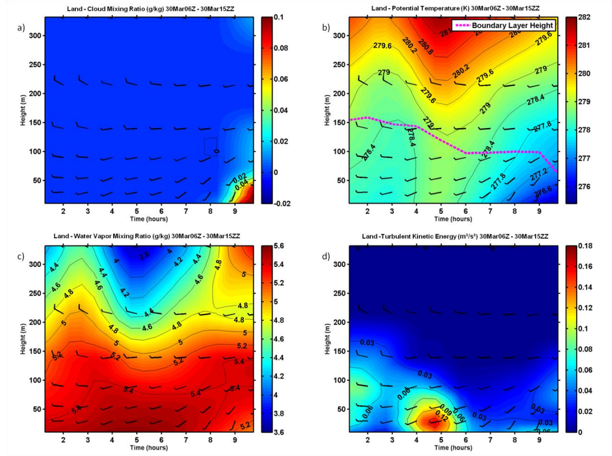
Figure 25. Contour plots along point L trajectory from 30 March/06Z to 30 March/15Z. a) q_c ; b) potential temperature with BL height; c) q_v ; d) TKE. Wind barbs represent the wind speed and direction of the flow in knots. The height level is up to 330m.
