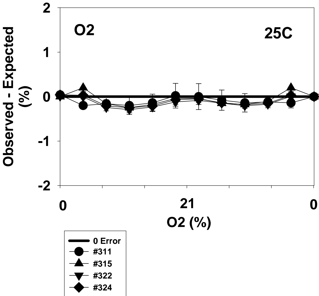
FIGURE 1A. O2 Accuracy: 25C Means and SDs, N=5-15
