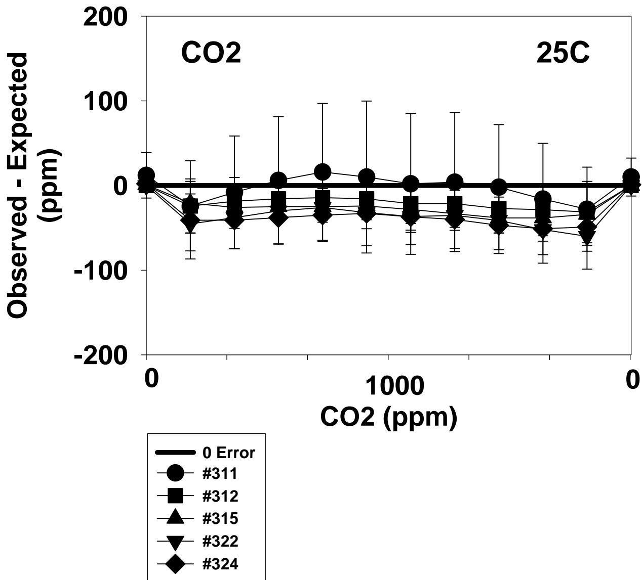
FIGURE 2A. CO2 Accuracy: 25C Means and SDs, N=5-15
