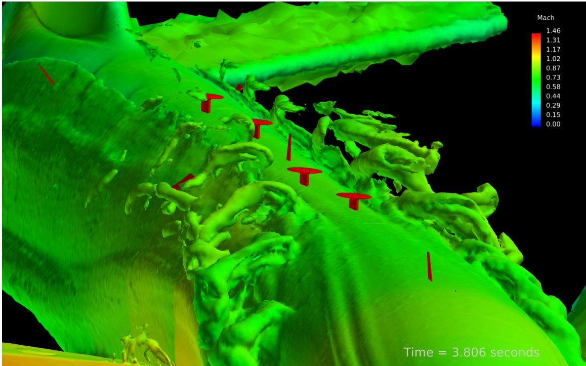
Figure 4.24: Rivet Joint with LCS ( AoA = 8^\circ ) – vorticity of 100 Hz colored by Mach number for high angle of attack study (antennas colored by red shown for reference locations only – not included in solution)
