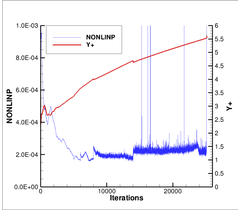
Figure 4.3: Examining Point 5 of the “steepest descent” method showing the residual and y^+ as a function of the number of iterations
