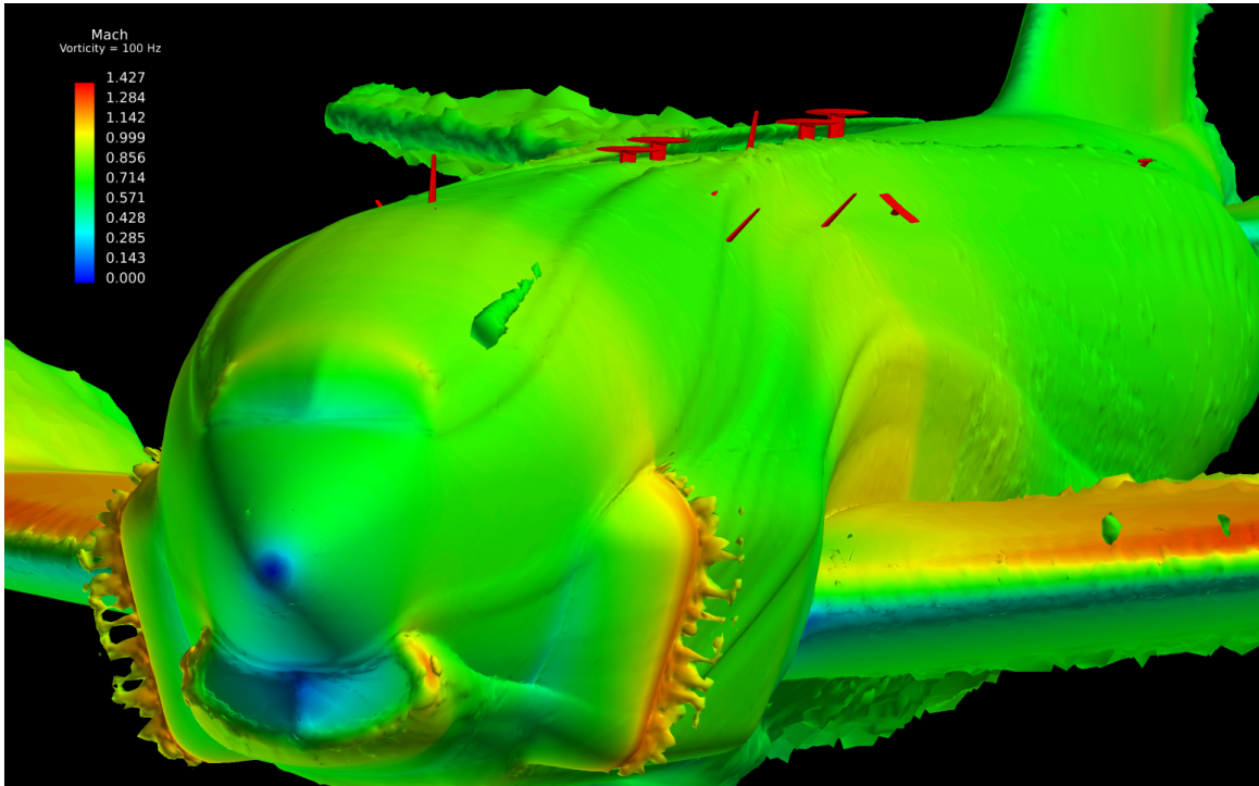
Figure 4.28: Combat Sent without LCS (AoA = 8^\circ ) – vorticity of 100 Hz colored by Mach number for high angle of attack study (antennas colored by red shown for reference locations only – not included in solution)
