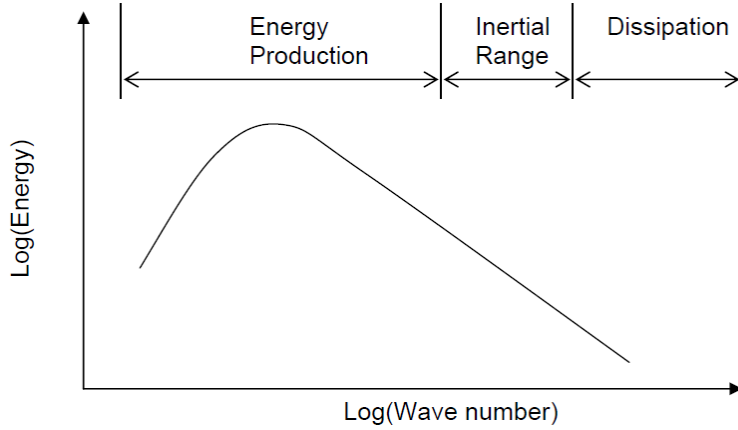
Figure 2.1: Turbulent energy spectrum [4]
