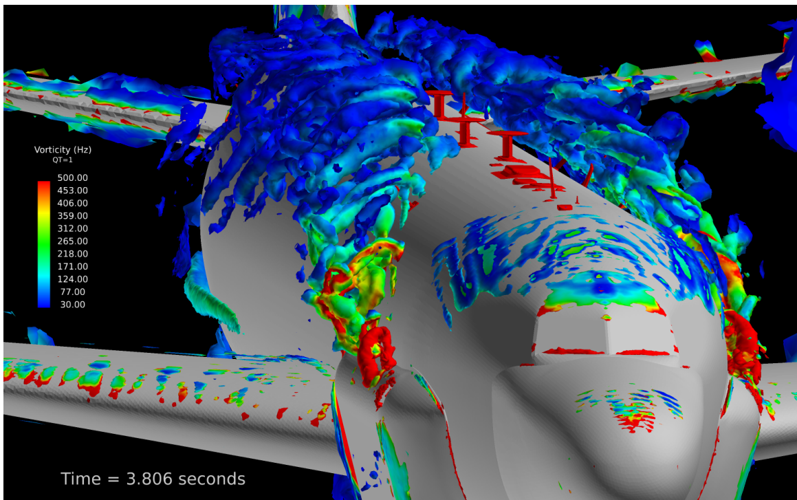
Figure 4.25: Rivet Joint with LCS (AoA = 8°) – Q-threshold of 1 colored by vorticity for high angle of attack study (antennas colored by red shown for reference locations only – not included in solution)
