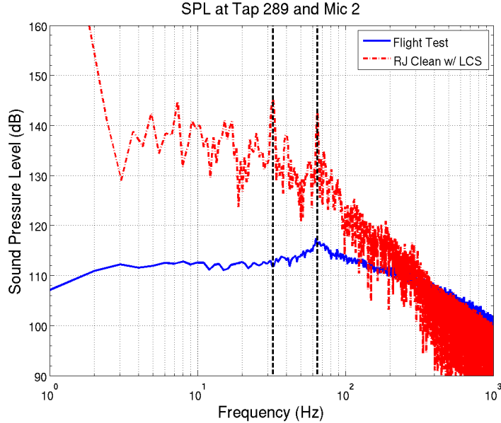
Figure 4.5: Comparison of computational and flight test derived acoustic spectrum for this case. The second to last microphone/tap comparison is placed in the aft end of the cheek where there is a pocket of separated flow and since exact microphone placement could not be determined, the acoustics would be expected to vary depending on where it is located in relation to this pocket. Additionally, placement of microphone 1 proves tricky as well as there is a fair amount of variance depending on how close the tap is to the exhaust. The jet flow exiting the exhaust seems to initially provide a pocket of “sheltered” flow immediately aft of the exhaust that manifests in lower SPL’s. Discounting the known error inherent to comparison with microphones 1, 4, and 5; the remaining two microphone locations exhibit similar acoustic trending despite under-predicting the OASPL by 9.7% and 13.4% respectfully. All in all, this is not completely unreasonable, but still does not provide adequate validation. This should be pursued further in any future research.
