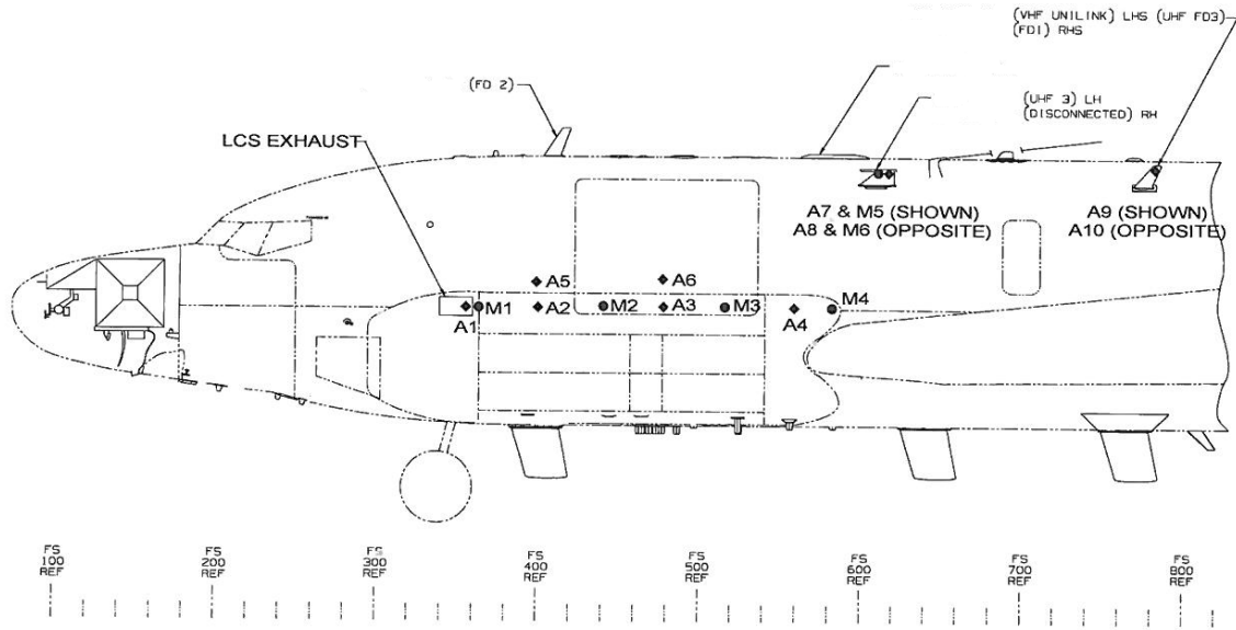
Figure 2.8: RC-135V/W accelerometer and microphone locations for flight testing perspective, the manufacturer specified vibration limit for the Sensor Systems, Inc. S65-8262-305 antenna is 10g. With louvers removed, the peak responses did drop to a range of approximately 3g to a little over 6g for the UHF3 and UHF5 antennas and a range of 3.6g to 12g for the Unilink antennas. [7]
