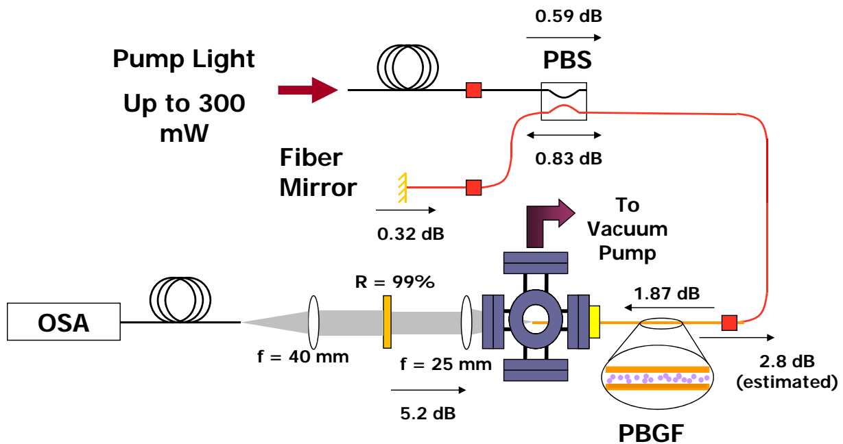
Figure 7.6 Initial setup for C_2H_2 -filled PBGF small quantum defect laser using a polarized cavity. Acetylene gas is contained in the 10- \mu\text{m} diameter hollow core of a \sim 1.5 -m long PBGF. The laser cavity is formed by the gold-coated fiber mirror connected to the polarizing beam combiner and the 99% reflective, plano dielectric mirror which functions as the laser output coupler. Pump light is polarized orthogonal to the polarization that the cavity supports and is coupled into the cavity through the polarizing beam combiner. The losses through various components are labeled in the figure.
