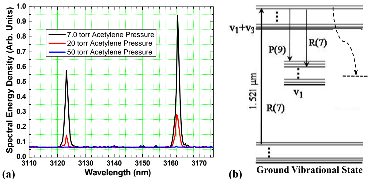
Figure 5.4 Spectrum and energy level diagram from the acetylene-filled HC-PCF laser. (a) The laser spectrum was taken at gas pressures of 7.0, 20, and 50 torr using a grating spectrometer with \sim 1 \text{ nm} resolution. While the relative energy density of the spectral features changes with pressure, no spectral shifts or additional features are observed. The two peaks correspond to transitions from the J = 8, \nu_1 + \nu_3 excited state to the J = 7 and J = 9, \nu_1 state, corresponding to wavelengths of 3123.2 nm and 3162.4 nm, respectively. (b) An energy level diagram showing the pertinent ro-vibrational transitions in the acetylene molecules. The dotted line represents potentially unobserved relaxation pathways.
