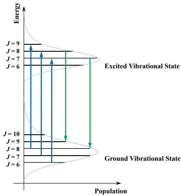
Figure 7.1 Energy level diagram illustrating the process of coherence generation with a small quantum defect laser. Pump transitions are indicated by the blue arrows pointing upwards while the laser transitions are indicated by the green arrows pointing downward and only occur between dipole-allowed transitions where population inversions exist. The rotational state population in each vibrational state follows a Boltzmann distribution (indicated by the gray dashed lines) owing to fast thermalization from collisions between molecules in the various rotational levels.
