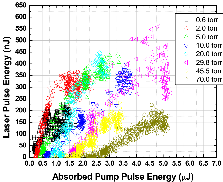
Figure 6.6 Plot of the measured mid-IR laser pulse energy as a function of absorbed pump pulse energy for a 1.46-m long, 18.75\text{-}\mu\text{m} pitch kagome-structured HC-PCF filled with various pressures of \text{C}_2\text{H}_2 gas. Plots of each pressure individually are shown in Appendix C. Reproduced from ref [34].
