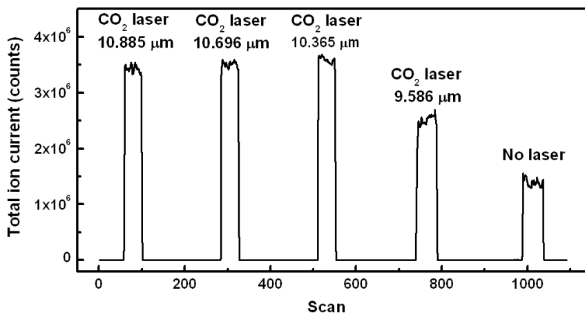
Figure 7.6 Chromatograph of the flame when irradiated by the CO_2 laser at 10.885, 10.696, 10.365, and 9.586 \mu m , and without laser irradiation.
