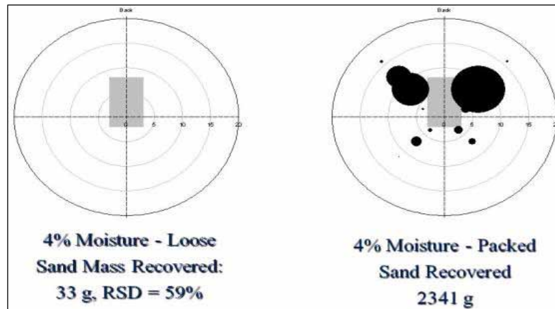
Figure 32. Application of 4% moisture (by weight) to sand, comparison of packed and loose bed surface.
