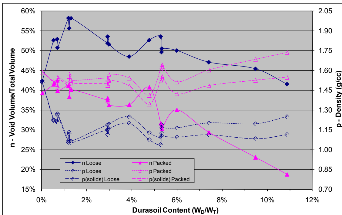
Figure 33. Open porosity and density vs. Durasoil content.
