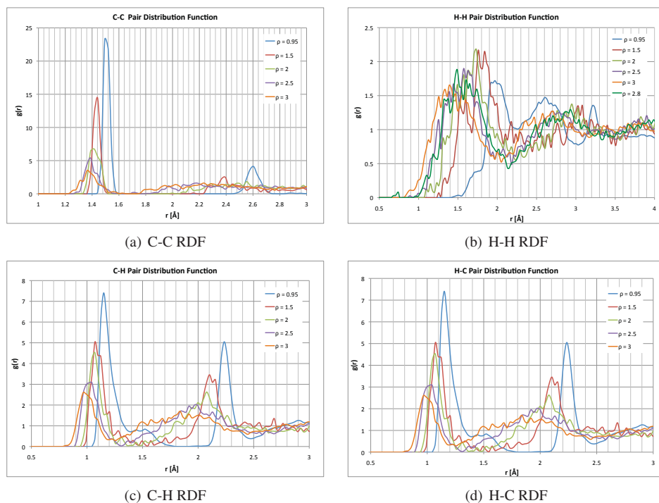
FIG. 4.2. Radial distribution functions for various pairs of nuclei. Each plot contains RDF data for densities of 0.95 , 1.5 , 2.0 , 2.5 , and 3.0 \text{ g/cm}^3 . The H-H RDF (b) also contains an RDF for 2.8 \text{ g/cm}^3 because compression to this density produces molecular hydrogen.
