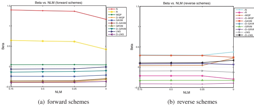
FIG. 4.3. \beta vs. NLM for the 20 vertex reordering schemes in Experiment 1. Results for the 10 forward schemes: N, R, WQP, D-WQP, GAVM, D-GAVM, GRVM, D-GRVM, LNG, and D-LNG are shown in (a). The results for the 10 reverse schemes: -N, -R, -WQP, -D-WQP, -GAVM, -D-GAVM, -GRVM, -D-GRVM, -LNG, and -D-LNG are shown in (b).
