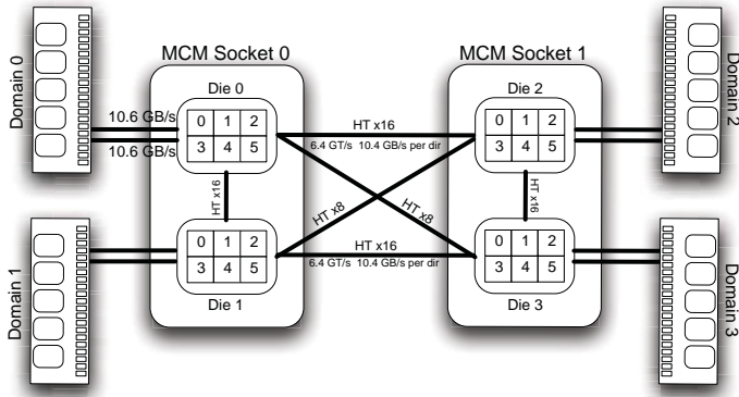
FIG. 1.1. Two AMD Opteron 6174 processors.
