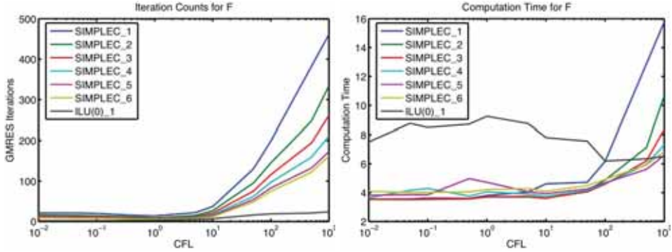
Fig. 6.6. Iteration count and computation time for Neumann series preconditioned by SIMPLEC applied to F .
