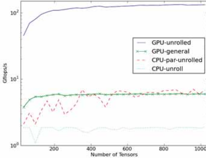
FIG. 6.2. Performance results for running SS-HOPM on sets of 4 th order 3-dimensional tensors with 128 starting vectors each. Note the y-axis is a log scale.
