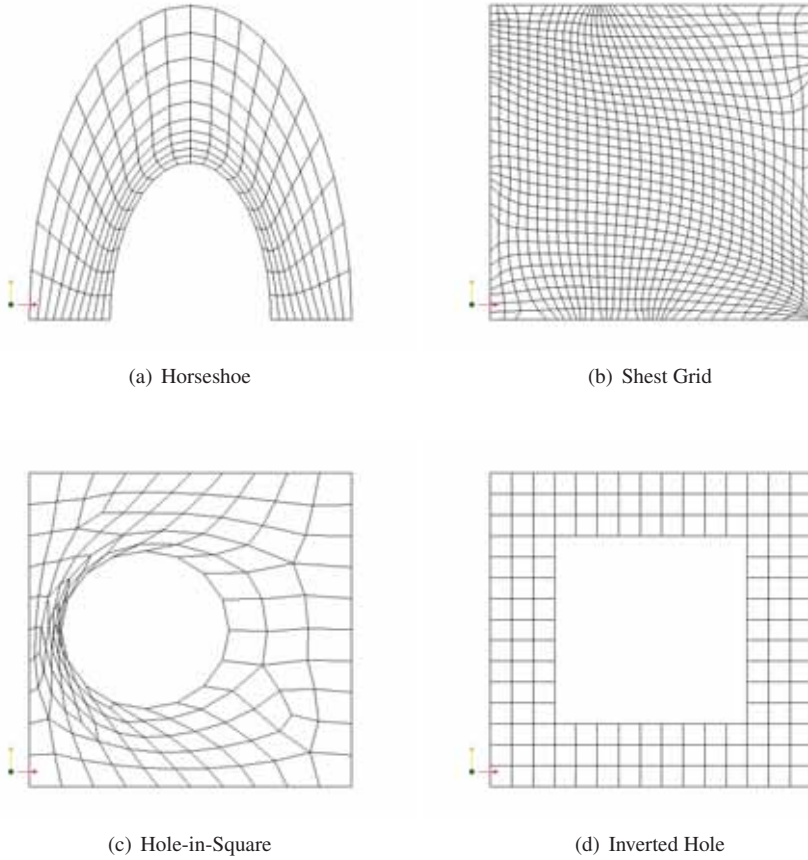
FIG. 3.4. All four meshes after optimization with f_{ShSzU} .
