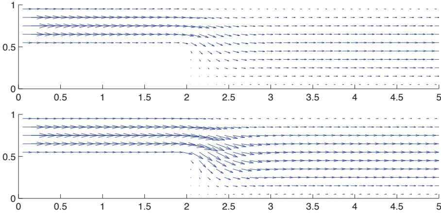
FIG. 5.2. Velocity plot of C^0 (2.19) (top) and SVP (3.8) (bottom) for the backward-facing step.
