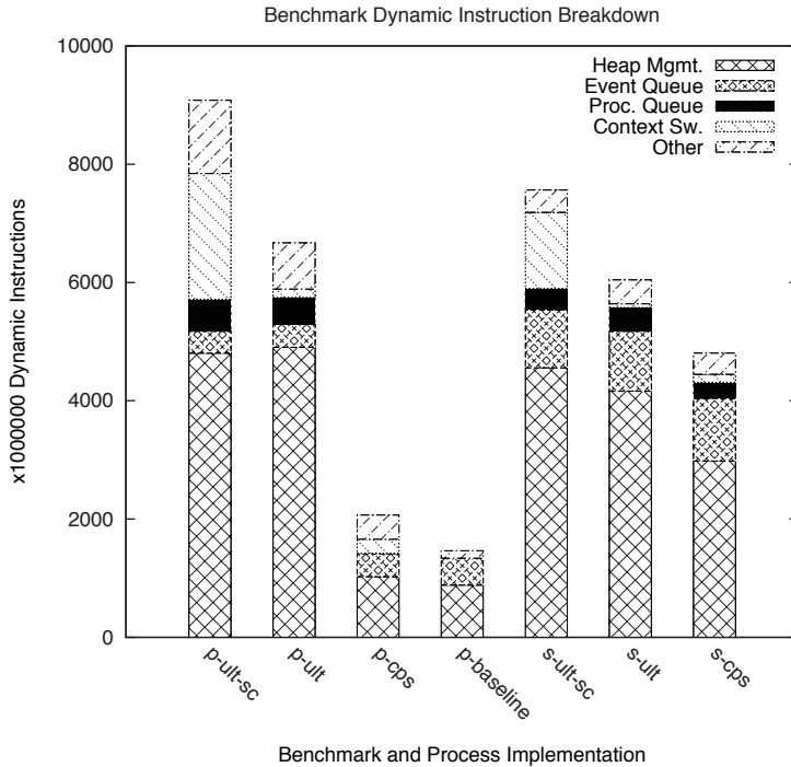
FIG. 6.2. Summary of dynamic instruction breakdown gathered with QSim profiler.
