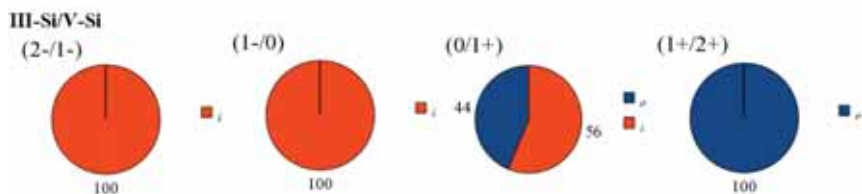
Fig. 5.4. Geometric relaxation occurrence percentages for the III-Si/V-Si.
