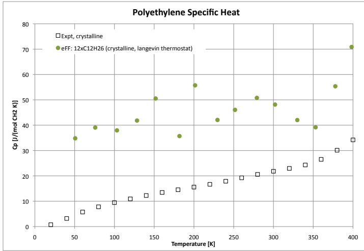
FIG. 4.5. The specific heat capacity of crystalline polyethylene. The green circles show data computed from constant volume heat capacity simulations computed using NVE with a Langevin thermostat. The data was converted to constant pressure heat capacity using the volume and compressibility parameters from [14]. The open black squares show experimental heat capacity data for polyethylene crystal taken from [9]
