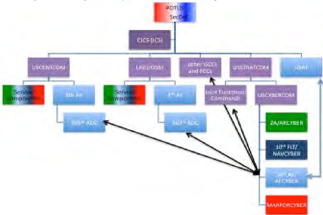
Figure 3 Course-Grained view of 24th AF interaction with AOCs’ Net Defense (NetD) and Network Operations (NetOps) Cells. The line from USAF to AFCYBER represents Administrative Control (ADCON) as well as Service-Specific NetOps.
