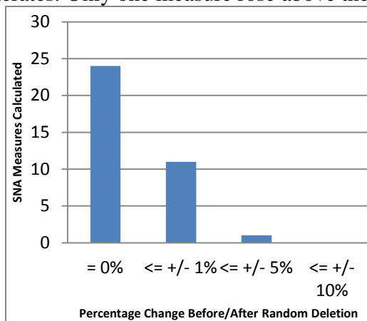
Figure 11 Effects for Random Deletion/Targeting of IT-Systems
