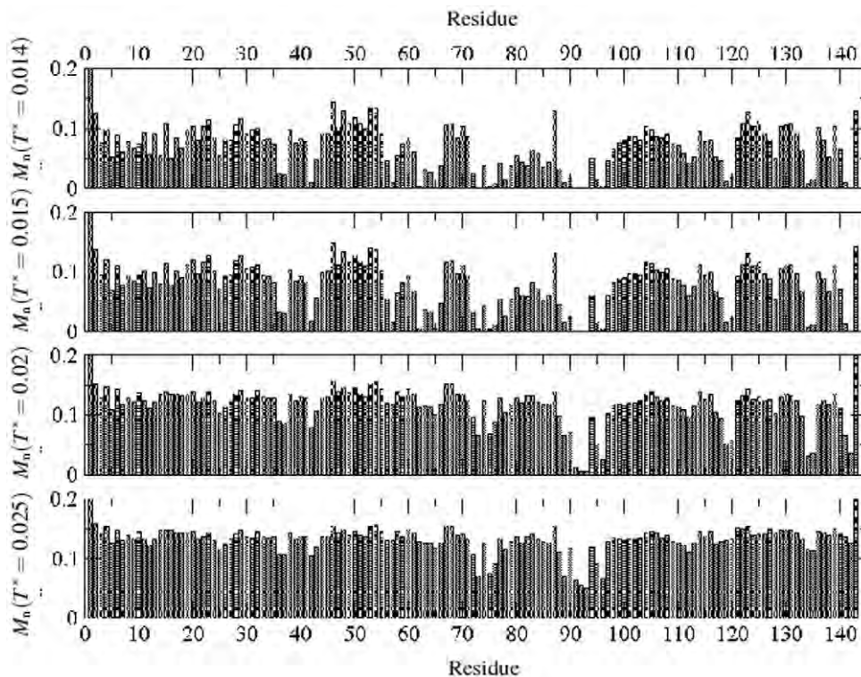
Figure 3. Mobility M_n of each residue (number of successful moves per unit time step) of the histone H2AX at temperatures T^* = 0.014, 0.015, 0.020, and 0.025 . The mobility of a residue is defined by the number of successful moves per unit MC time step. With exceptions the mobility profile of the residues follows the energy profile relatively closely where the lower segmental energy differences translate into lower segmental mobility. Interestingly, some residues, 42E and 57E, show a low mobility despite their positive energy. doi:10.1371/journal.pone.0032075.g003
