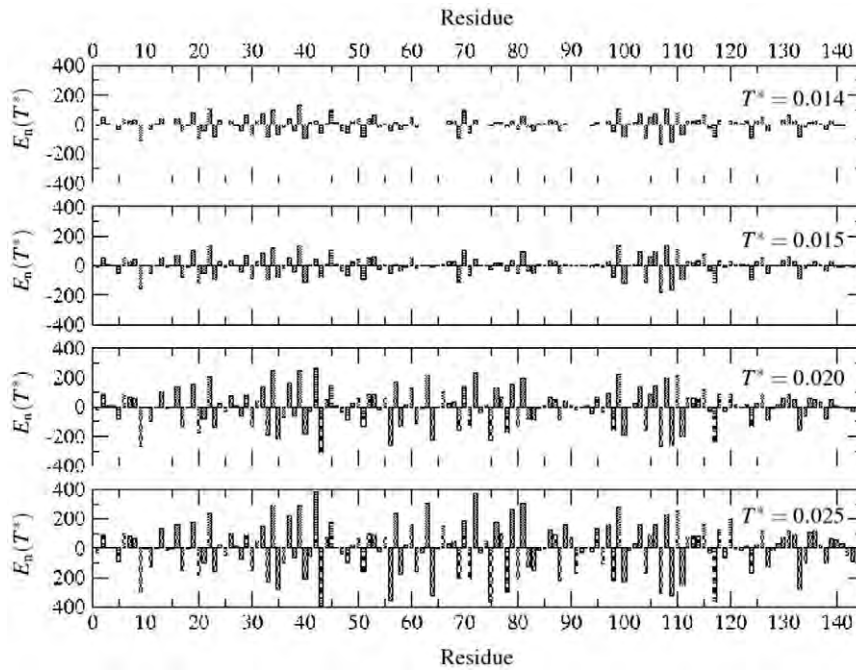
Figure 2. Energy E_n of each residue of histone H2AX at normalized temperatures T^* = 0.014, 0.015, 0.020, and 0.025 . The energy of a residue is its interaction energy with neighboring residues within the range of interaction. The magnitude of the repulsive and the attractive energy and their differences in consecutive segments increases with temperature which is manifested in the global (coil-to-globule) structure of the protein. At low temperatures ( T^* = 0.014, 0.015 ), residues with the lowest mobility consist of 36R, 37K, 57E, 62E, 65E, 72R, 73D, 75K, 76K, 78R, 89R, 90N, 91D, 92E, 93E, 95N, 96K, 119K, 120K, 134K, 135K, 141Q and 142E. Nearly all the electrostatic residues (D, E, K, R) along with a few polar groups (Q, N) act as anchor/seed for segmental aggregation. doi:10.1371/journal.pone.0032075.g002
