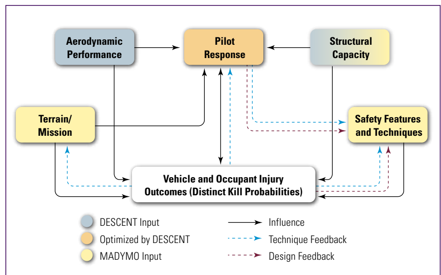
Figure 2 Data Flow with MADYMO-Based Occupant Loading Analysis
