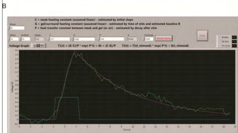
Figure 11. Thermister measurements after high power sonication at A) the surface of the phantom and B) through 2'' of soft tissue
