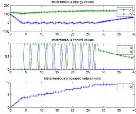
Fig. 2. Optimal solution under r(0) = 100 , b(0) = 120 , c_1 = 30 , c_2 = 10 , k = 0.05 , \beta = 0 , T = 40 , B = 150 with the constraints r(t) \geq 0 and b(t) \leq B .
