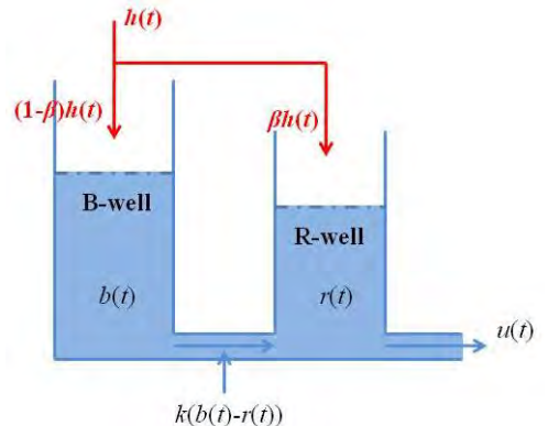
Fig. 1. Kinetic Battery Model modified to include recharging
