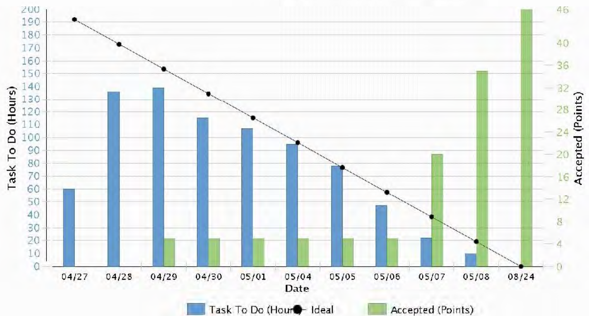
Iteration Burndown
