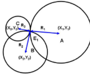
Figure 3 - Triangulation typically used in cooperative localization when multiple access points are available
