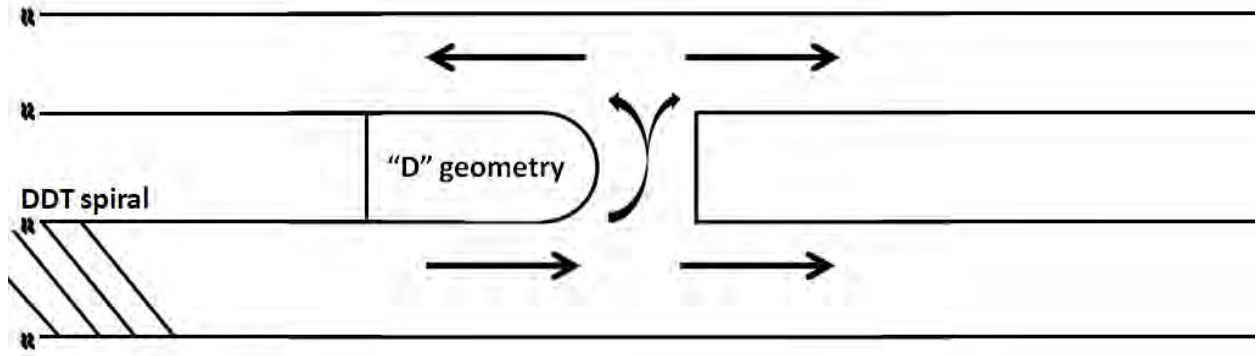
Figure 15. Two-tube mid-mid crossover configuration.
