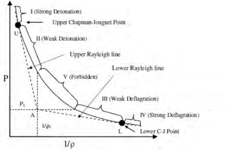
Figure 4. Hugoniot curve and Rayleigh lines 14,16
