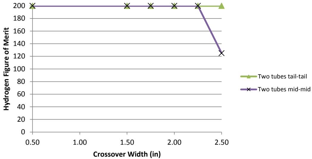
Figure 41. Hydrogen figure of merit for tail-tail and mid-mid configurations
