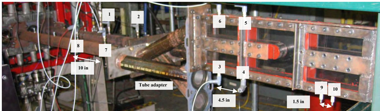
Figure 18. Two-tube configuration with engine head on the left side and crossover section on the right. Ion probes are numbered throughout.
