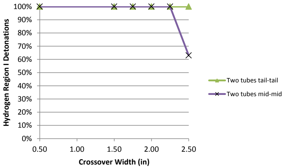
Figure 42. Hydrogen Region I detonations for tail-tail and mid-mid configurations
