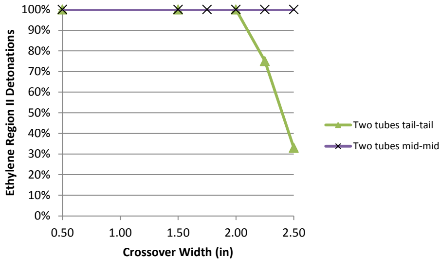
Figure 35. Region II ethylene detonations for tail-tail and mid-mid configurations
