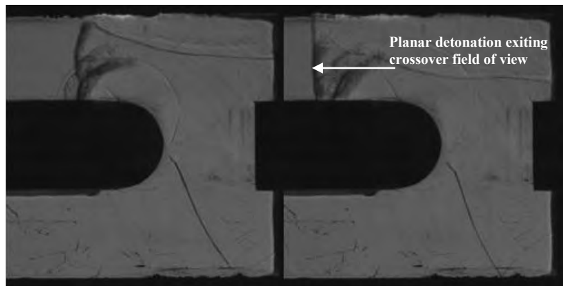
Figure 48. Mid-mid configuration hydrogen-air detonation with 2.0 in crossover width reinitiates, recouples across the entire secondary detonation tube and becomes planar in secondary tube prior to leaving the visible section of the crossover
