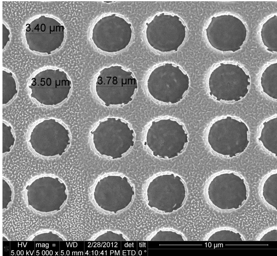
Figure 65. SEM micrograph of the center of a hybrid photonic crystal-multilayer structure at 5000 \times magnification. The Ge-Ag-Ge-Ag (4-12-270-200 nm) multilayer was deposited on a Si substrate. The square array of circular holes was milled into the multilayer using a focused ion beam system.
