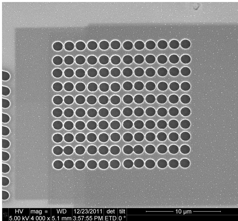
Figure 58. SEM micrograph of a hybrid photonic crystal-multilayer (Ag-Ge-Ag) on a silicon substrate. Ag and Ge layers were deposited via a High Power Impulse Magnetron Sputtering (HIPIMS) technique with dimensions 6-240-160 nm. The hole array was milled into the multilayer using focused ion beam (FIB) milling. Micrograph was taken from surface normal.
