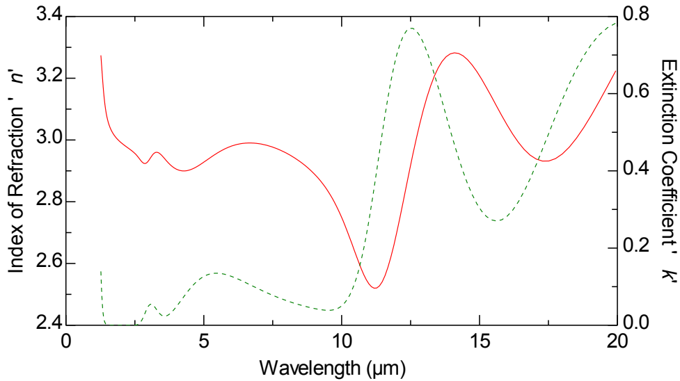
Figure 32. Calculated complex index of refraction, n (red) and k (green), for a Ge layer deposited via a High Power Impulse Magnetron Sputtering (HIPIMS) technique.
