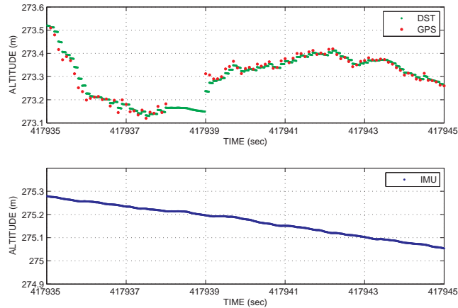
Figure 74: Altitude Outage
