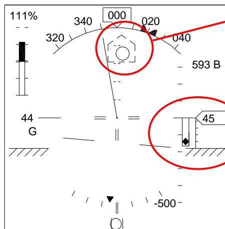
Figure A-13: BOSS Display as Flown on the NASA-Ames Vertical Motion Simulator.
