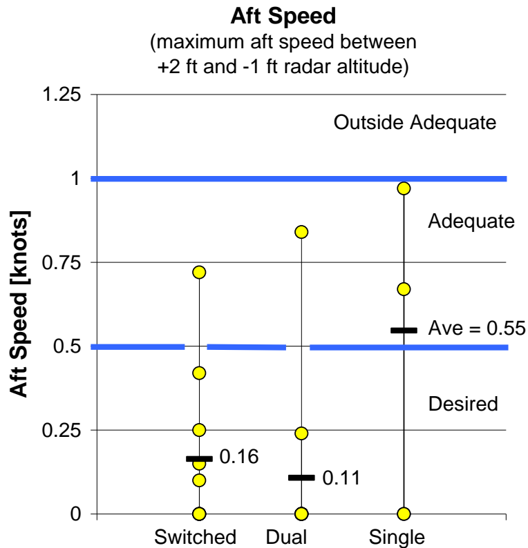
Figure C-20: Aft Speed.
