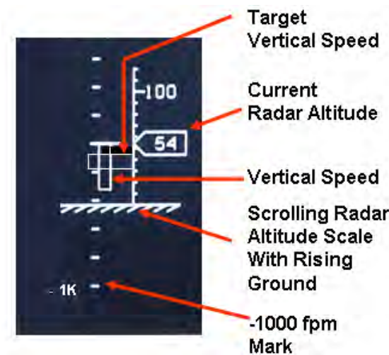
Figure C-11: Combined Altimeter and Vertical Speed Indicator with Target Vertical Speed Symbol Used for the Landing Maneuver.
