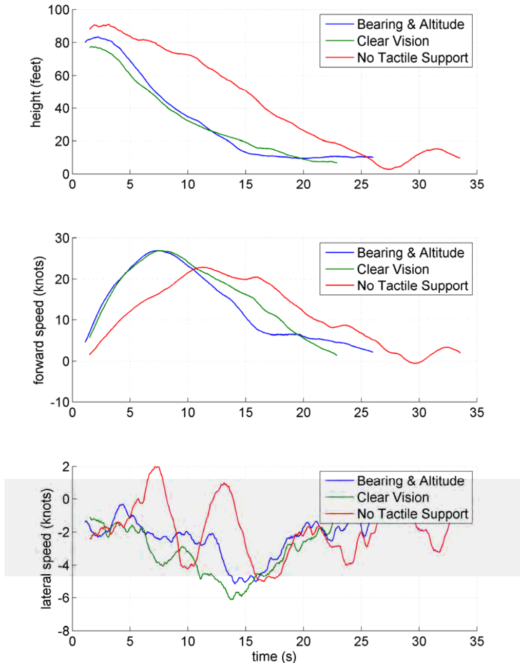
Figure B-5: Recorded Height-Above Terrain (Upper Plot), Forward Speed (Middle), and Lateral Speed (Bottom) Recorded During the Last Landing Maneuver in Three Conditions (Bearing and Altitude Information Presented on Tactile Display, Clear Vision, and No Tactile Support).
