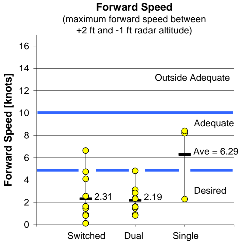
Figure C-19: Forward Speed.
