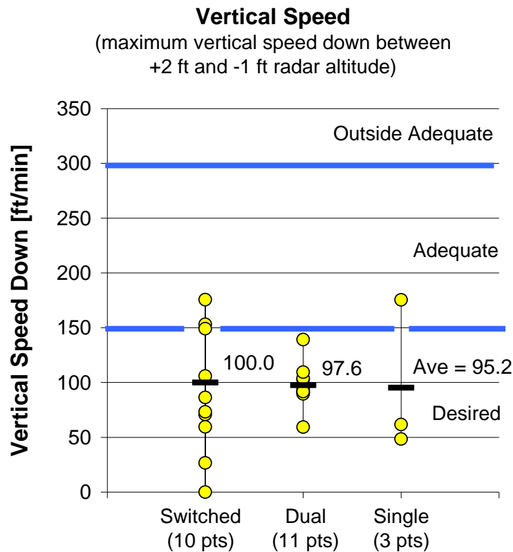
Figure C-17: Vertical Speed.
