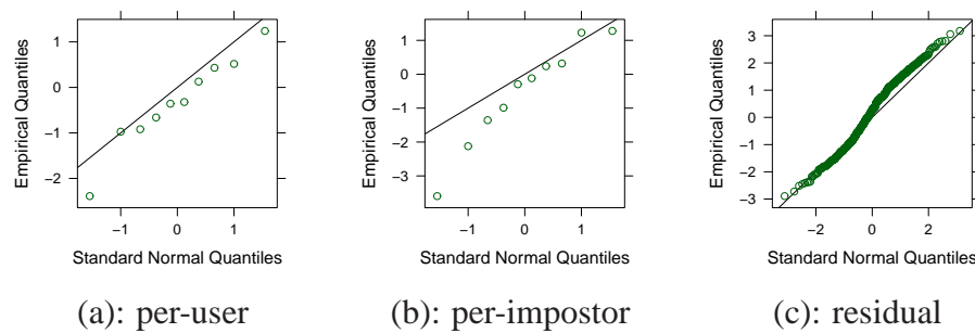
Figure 3.6: QQ -plots for validating LMM predictions from the example evaluation. The left panel assesses the Normality of per-user effects; the middle panel assesses per-impostor effects; the right panel assesses residual effects. Per-user and per-impostor deviations meet expectations except for one or two low outliers. Residuals show a slightly heavy tail.
