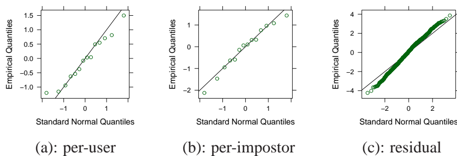
Figure 4.8: QQ -plots for validating LMM predictions from the benchmark evaluation. The left panel has per-user deviations from Normality; the middle panel has per-impostor deviations; the right panel has residual deviations. Per-user and per-impostor deviations meet expectations. Residuals are somewhat heavy tailed.
