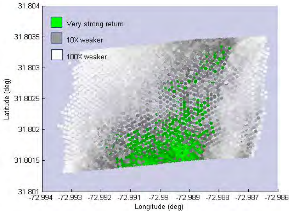
Fig. 4. Geo-registered fluorescein dye returns from a single flight pass. From B. Concannon’s report.
