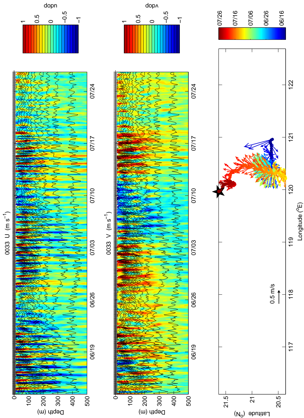
Figure 2: As in Figure 1, but for Spray 33 which is obtaining profiles along 20.6^{\circ}\text{N} and 120.25^{\circ}\text{E} .
