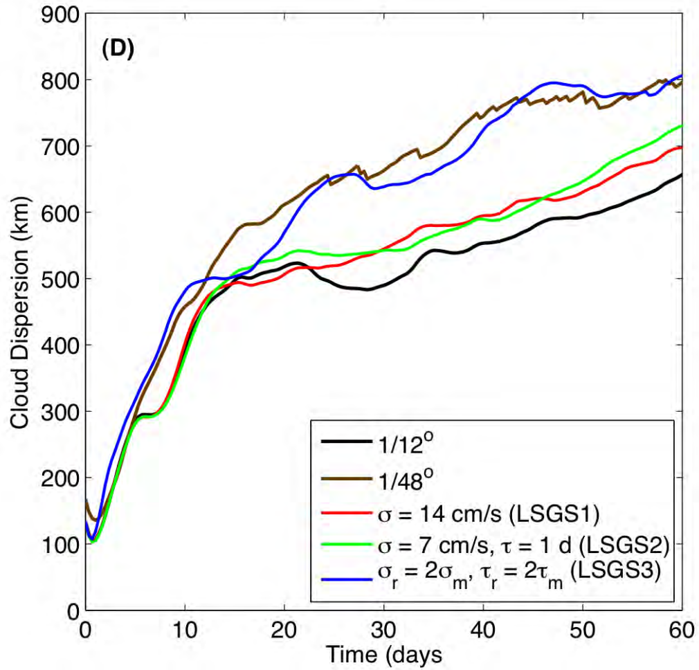
Fig. 4: Comparison of second moment of particle position variance (cloud spreading) from 1/12° (black) and 1/48° (brown) HYCOM output and those from LSGS-1, LSGS-2 and LSGS-3. Note that only LSGS-3 leads to a similar cloud spreading as in the submesoscale-containing 1/48° simulation.
