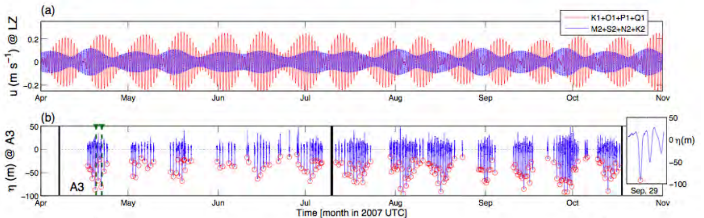
Fig. 2: (a) Semidiurnal (blue) and diurnal (red) predicted tidal component at Luzon Strait (122°E, 21°N). (b) Internal waves observed at A3. Vertical blue lines identify high frequency nonlinear internal waves detected at A (upper and lower bounds of the leading wave in a wave-train, illustrating intermittency of nonlinear internal waves and relationship to semidiurnal tidal forcing).
