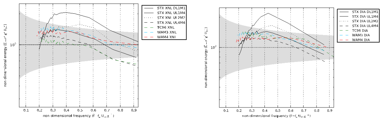
Fig.1. Total wave energy (dimensionless) versus dimensionless peak frequency, for different source functions as indicated in the legends. The dependences are normalised by the observational parameterisation of Babanin and Soloviev (1998a), which therefore equals unity in Figure, with shaded areas showing 95% confidence limits. Green lines indicate Tolman and Chalikov (1996) source functions, blue lines WAM3 and red lines WAM4 physics, respectively. Suit of black lines correspond to Donelan et al. (2006) wind input in the Tsagareli et al. (2010) version and to the four versions of Babanin and Young (2005) dissipation, following Rogers et al. (2011). UL4M4 is the preferred version for the subsequent modelling. (Left) Exact nonlinear term is used. (Right) DIA nonlinear-interaction term is used
