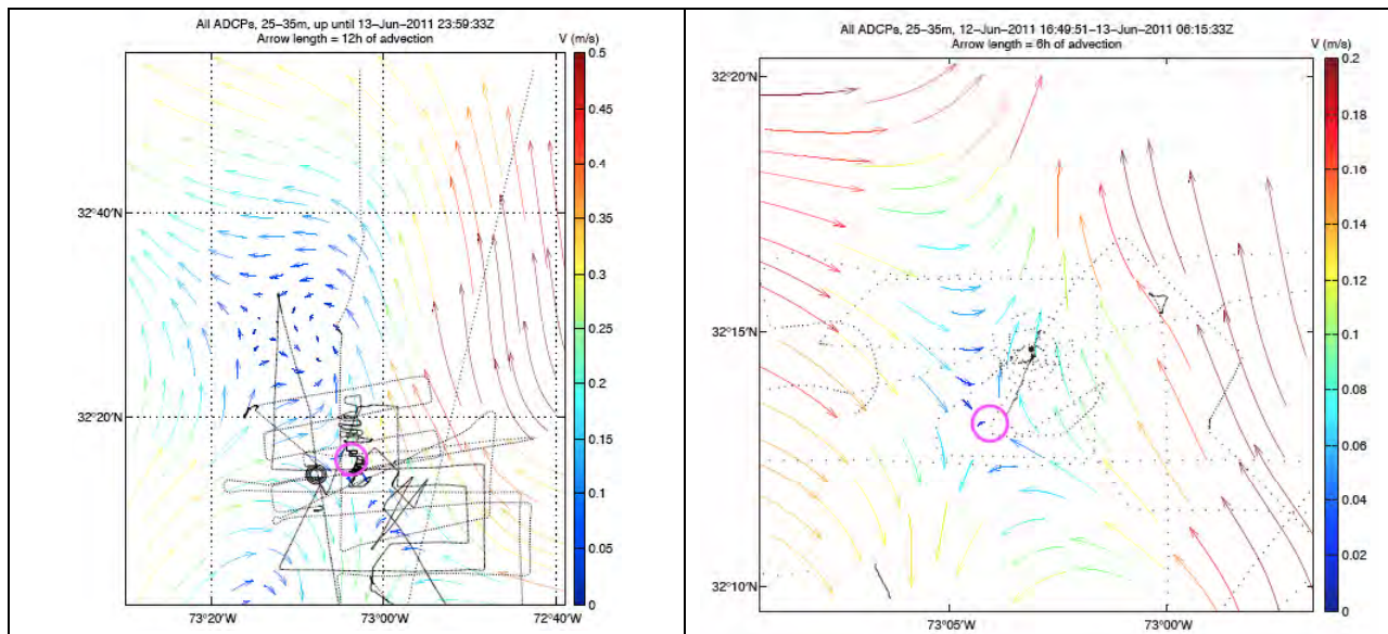
Figure 2. Objective maps of near-surface current on a 60 nm scale (left) and 10 nm scale (right) show a classic stagnation point at the magenta circle, with currents converging from the northwest and southeast, and diverging to the northeast and southwest.
