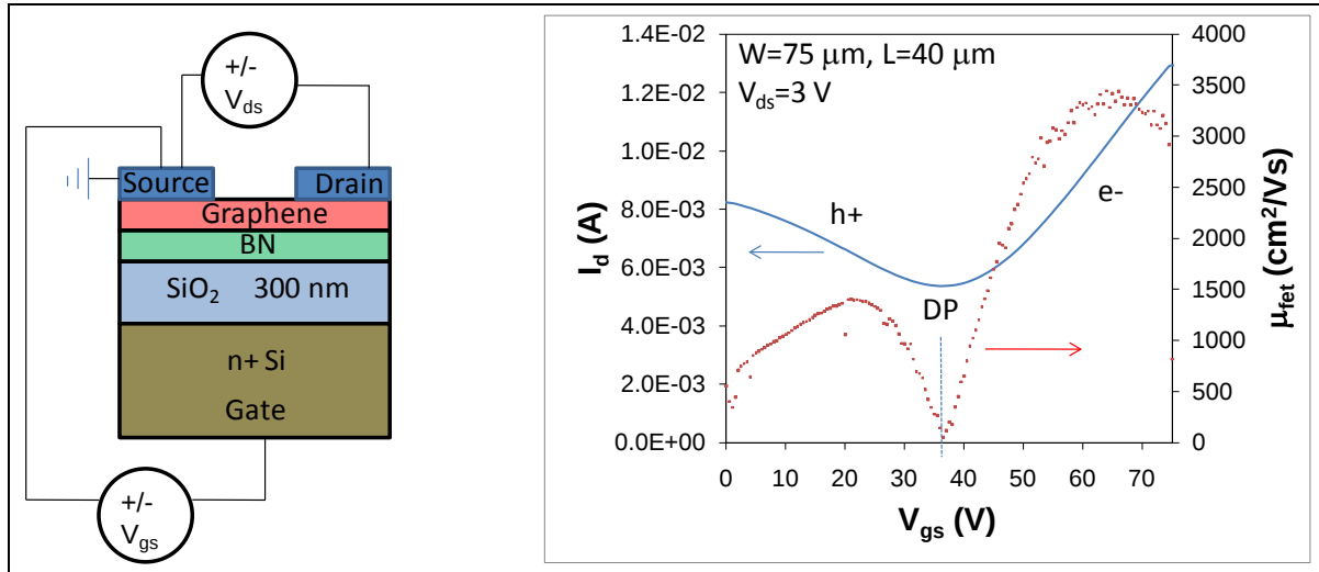
Figure 26. (Left) Schematic of graphene-on-BN transistor and biasing and (right) measured transfer characteristics and field-effect mobility.
