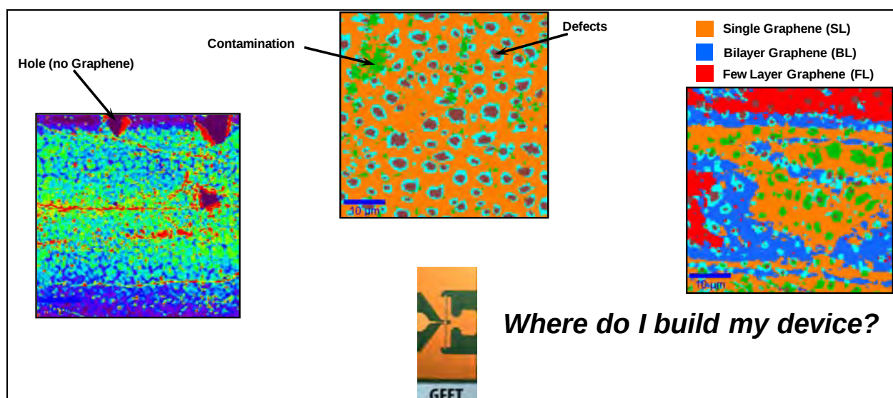
Figure 23. 50x50 \mu\text{m} Raman maps of graphene indicating holes, contamination, regions of high defects, and layer number. It is evident that certain regions are not suitable for device fabrication.
