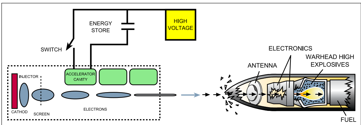
Figure 8. Charged-Particle Beam (CPB) Concept
