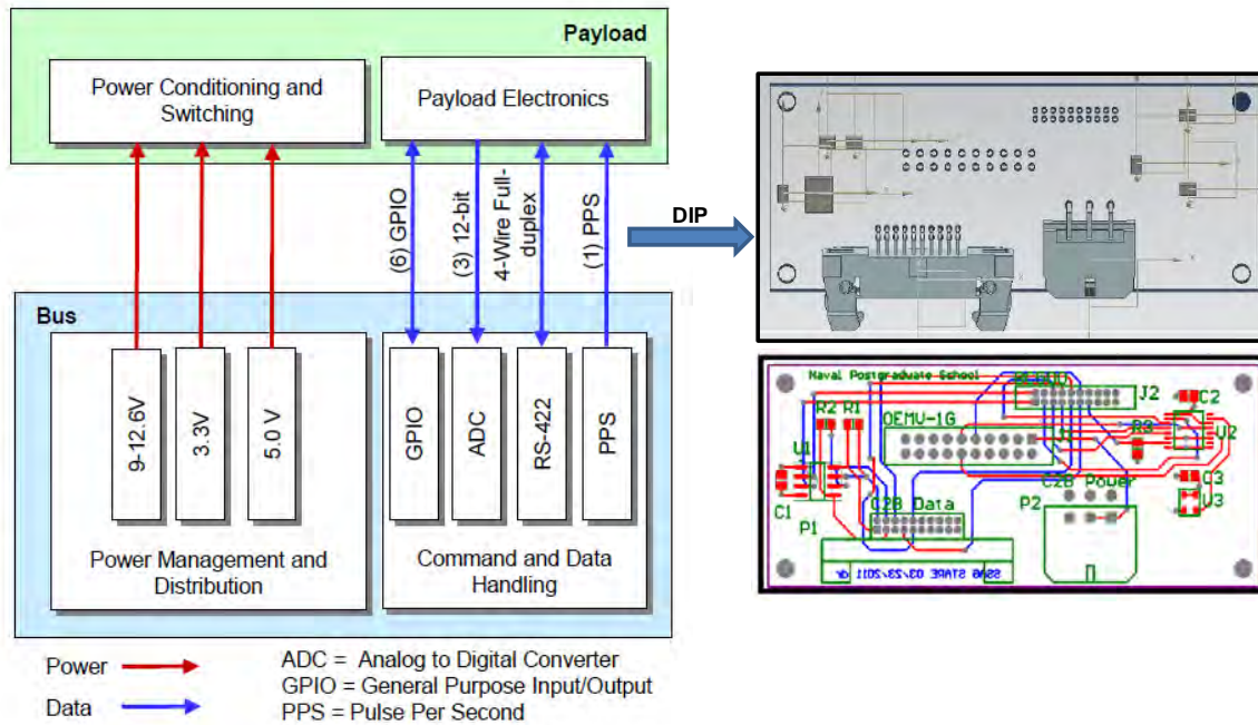
Figure 21. Data Interface and Power Board to Integrate STARE Payload to C2B (After NanoSat Engineering, 2011, Pg.40 and Riot et al., 2011 Slide 73)
