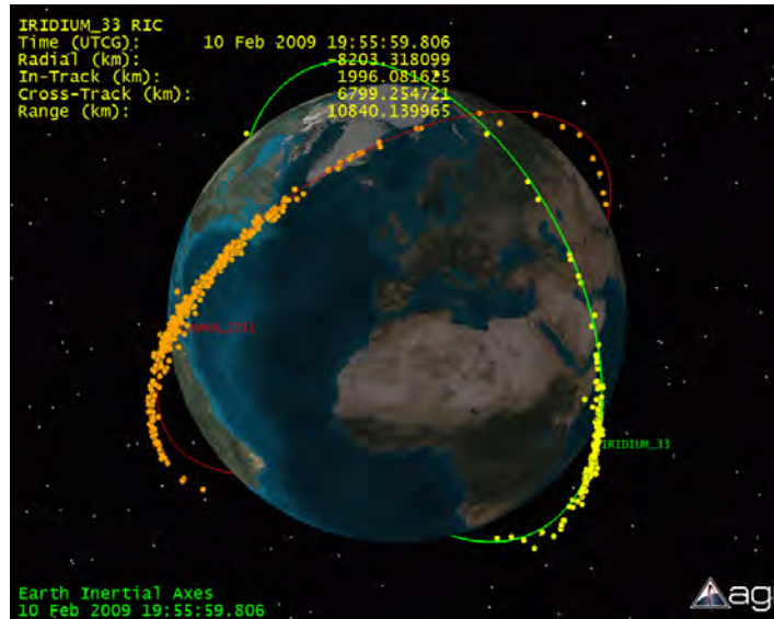
Figure 7. View of Iridium 33 and Cosmos 2251 orbits and debris 180 minutes post-collision (From Kelso, 2009)
