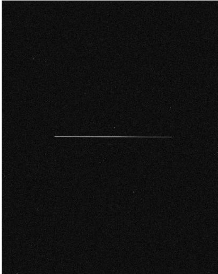
Figure 30. Simulated image for an Iridium 16 conjunction (From Riot, Olivier, Perticia, Bauman, Simms, & De Vries, 2010 p. 59)
