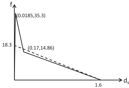
Fig. 14. Tri-linear bridging law is indicated by solid line. The dotted line is the linear softening law in Fig. 3. The areas under the force–displacement diagram for both laws are the same.
