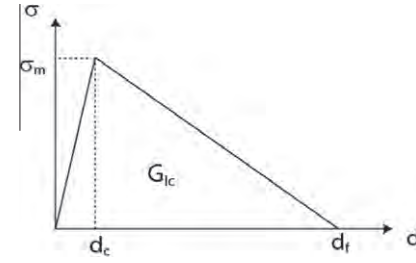
Fig. 9. Traction–separation law for the cohesive element.
