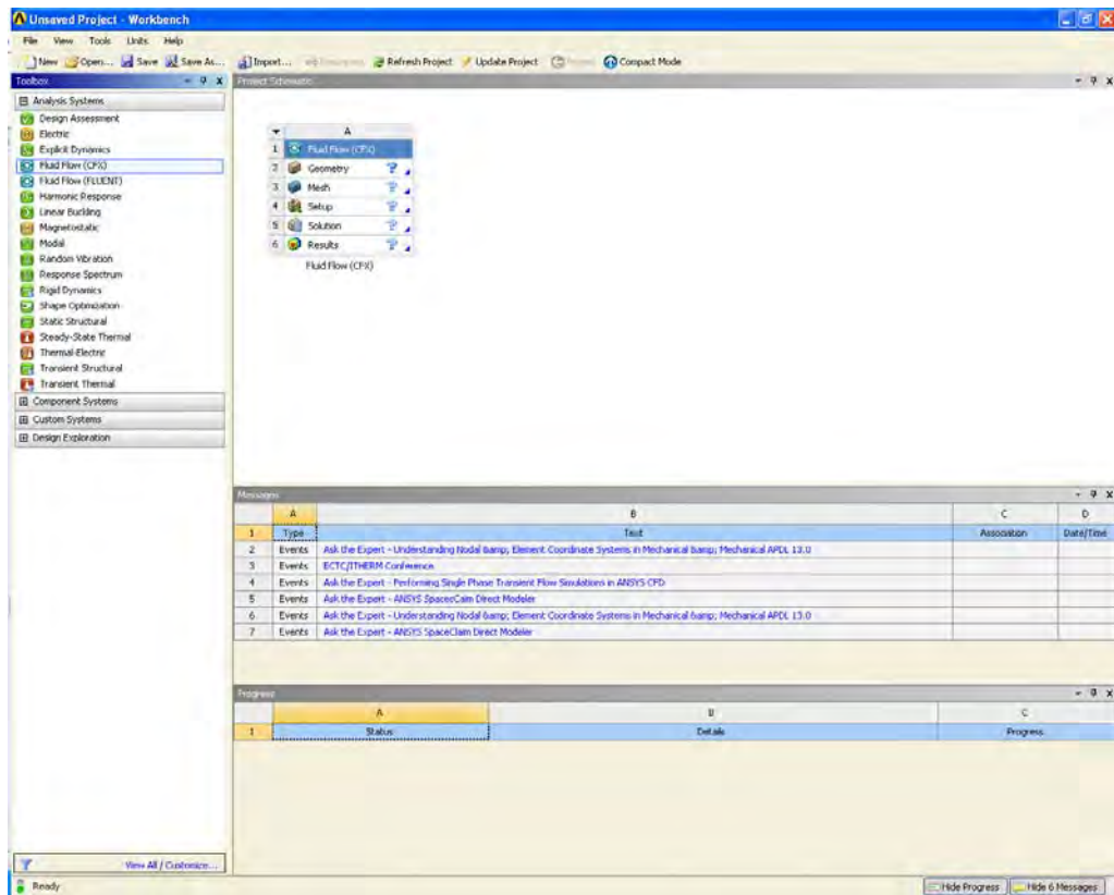
Figure 6. ANSYS GUI.
