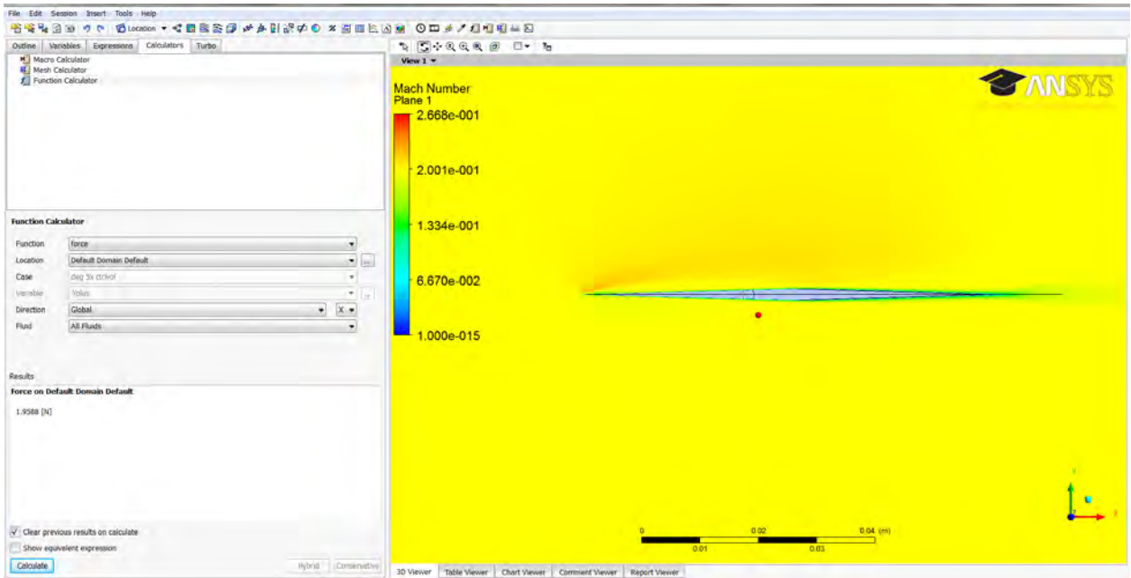
Figure 19. Function Calculator.
