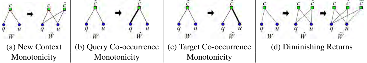
Figure 2: (a) New Context Monotonicity (NCM): joint observations in a new shared context increase similarity. (b) Query Co-occurrence Monotonicity (QCM): new query observations in a shared context increase similarity. (c) Target Co-occurrence Monotonicity (TCM): new target observations in a shared context increase similarity. (d) Diminishing Returns (DR): incremental similarity gains due to subsequent observations decrease as items share more contexts.
