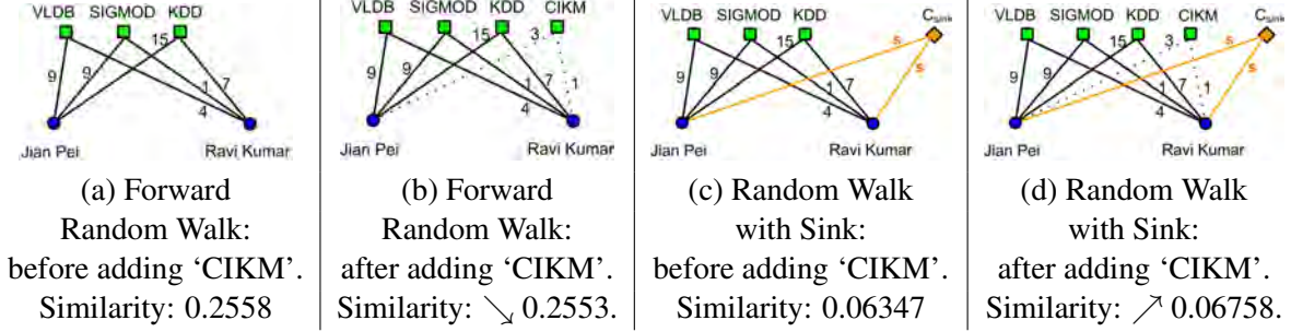
Figure 1: The comparison of the Forward Random Walk (FRW) and our proposed Random Walk with Sink (RWS) method. In (a) and (b), the new context ‘CIKM’ decreases the FRW similarity between Jian Pei and Ravi Kumar, which is counterintuitive and violating the Axiom 1 ‘New Context Monotonicity’. In (c) and (d), the same context increases the RWS similarity with the parameter s = 100 , showing that RWS satisfies the Axiom 1.
