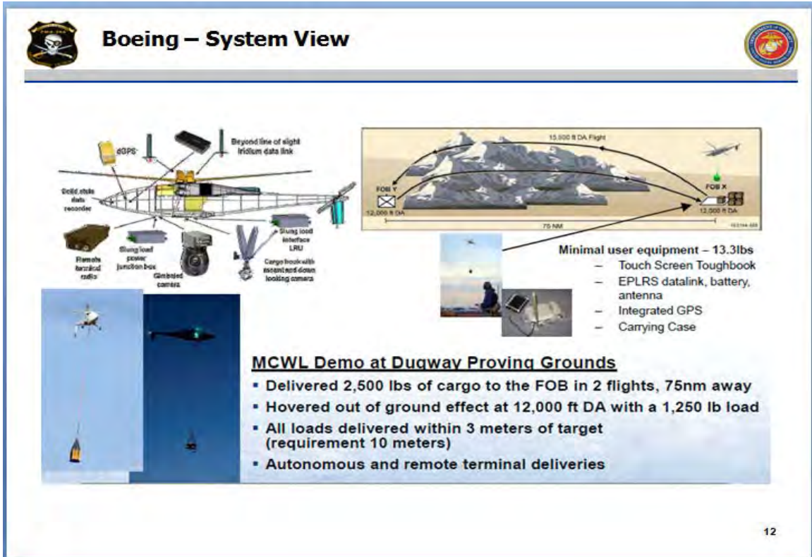
Figure 13. Boeing System View (From: E. N. Pratson, personal communication, June 12, 2011)
