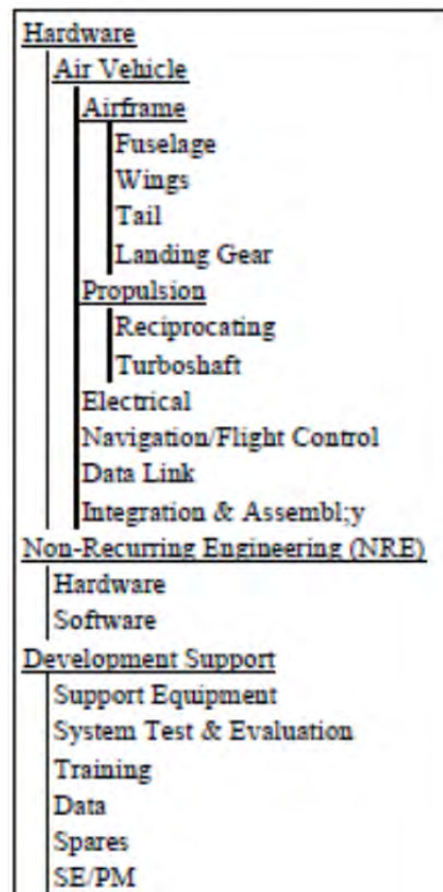
Figure 1. UAS Work Breakdown Structure (From Horak, Harbour, & Holcomb, 2007, p. 3)
